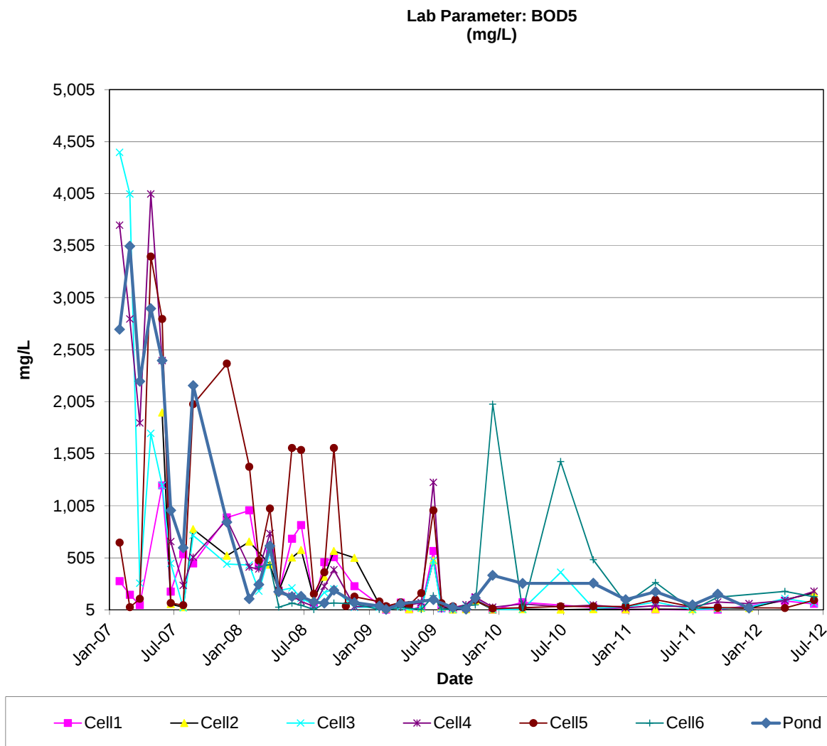
Figure 4-10 BOD5 of Leachate
