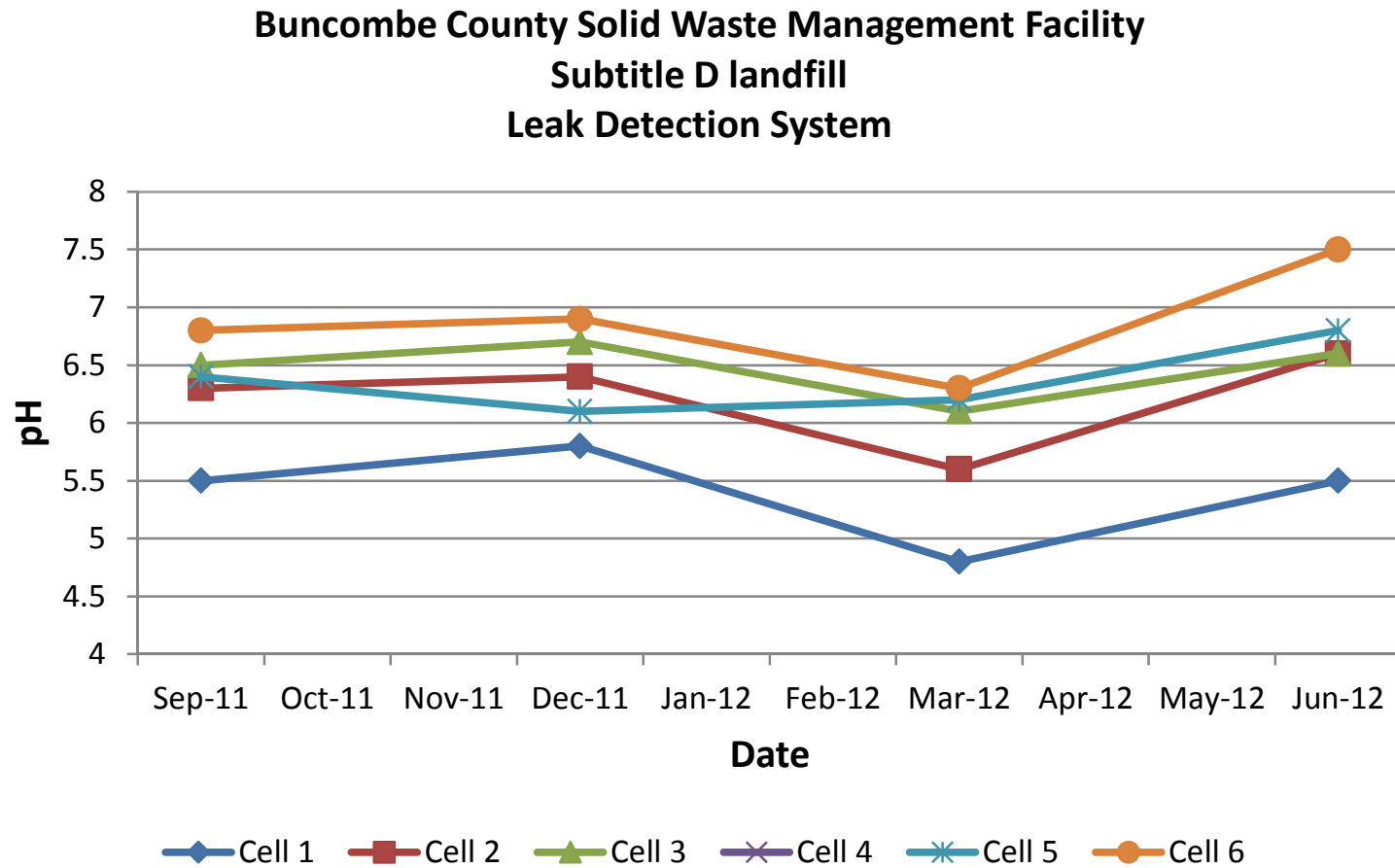
Figure 4-2 pH
