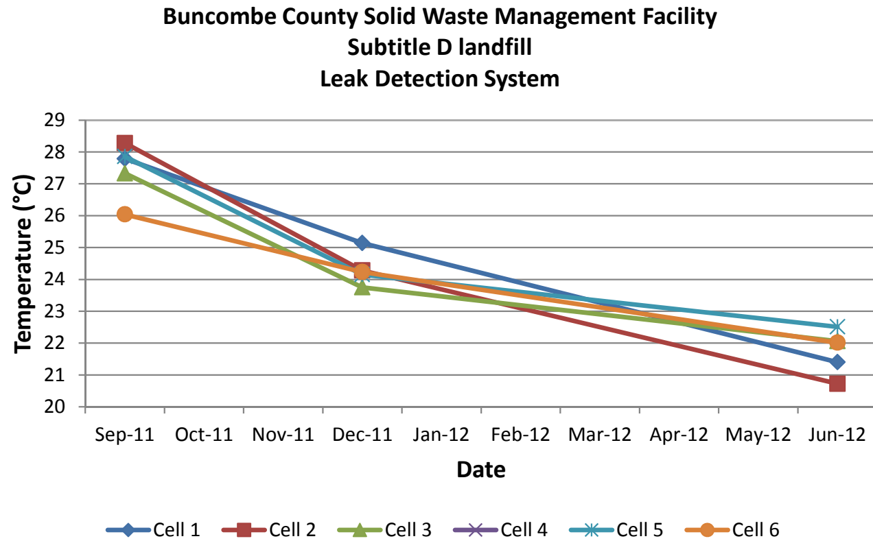
Figure 4-3 Temperature
