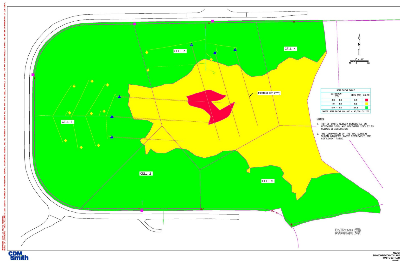
Figure 4-19 Settlement in Cells 1-5 since November 2010
