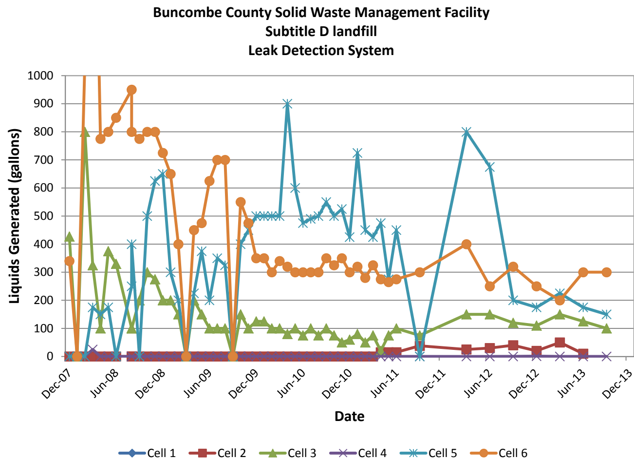
Figure 4-1 Monthly Leak Detection Volumes
