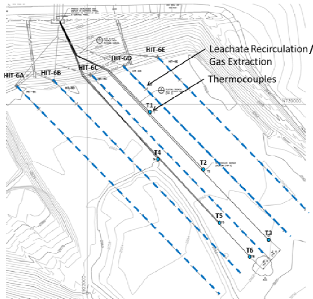
Figure 4-20 Temperature Sensors in Cell 6
