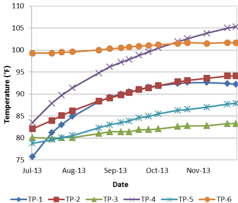
Figure 4-21 Waste Temperature Readings in Cell 6
