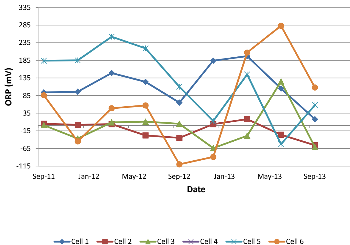
Figure 4-4 Oxidation Reduction Potential
