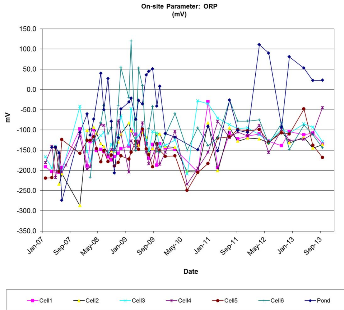
Figure 4-13 ORP of Leachate
