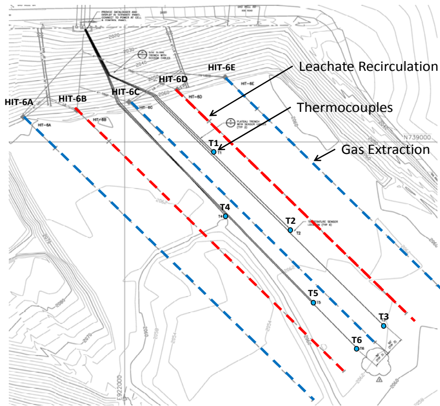
Figure 6-2 An Option Discussed at the Stakeholders Meeting for Cell 6 HIT Operation
