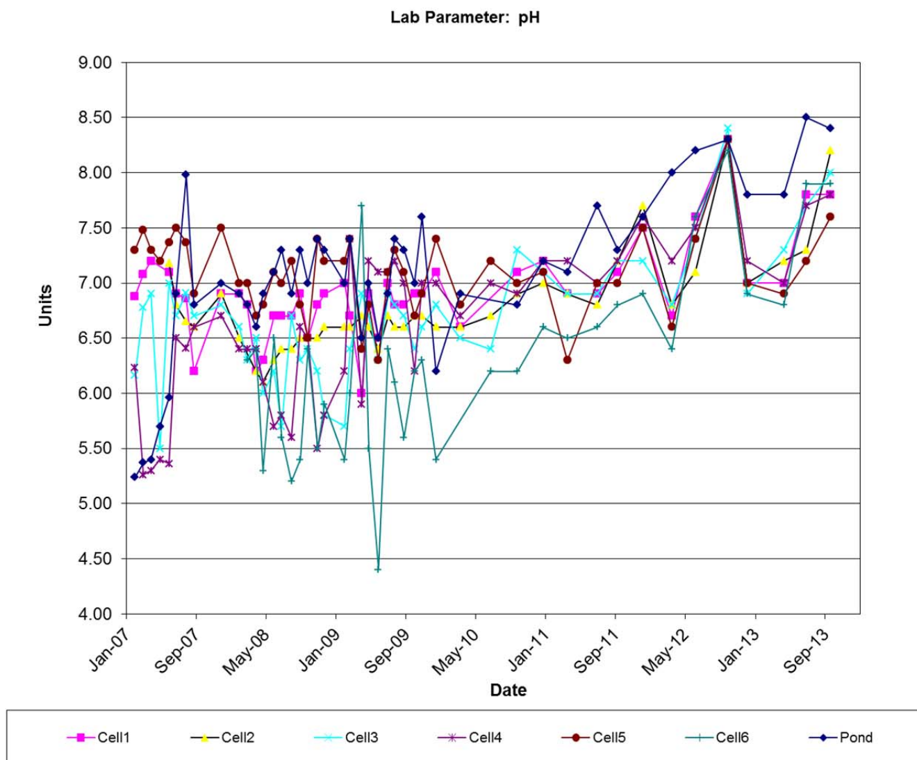
Figure 4-12 pH of Leachate
