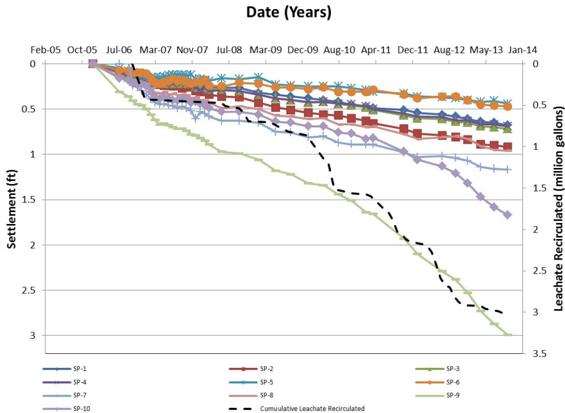
Figure 4-18 Cumulative Settlement
