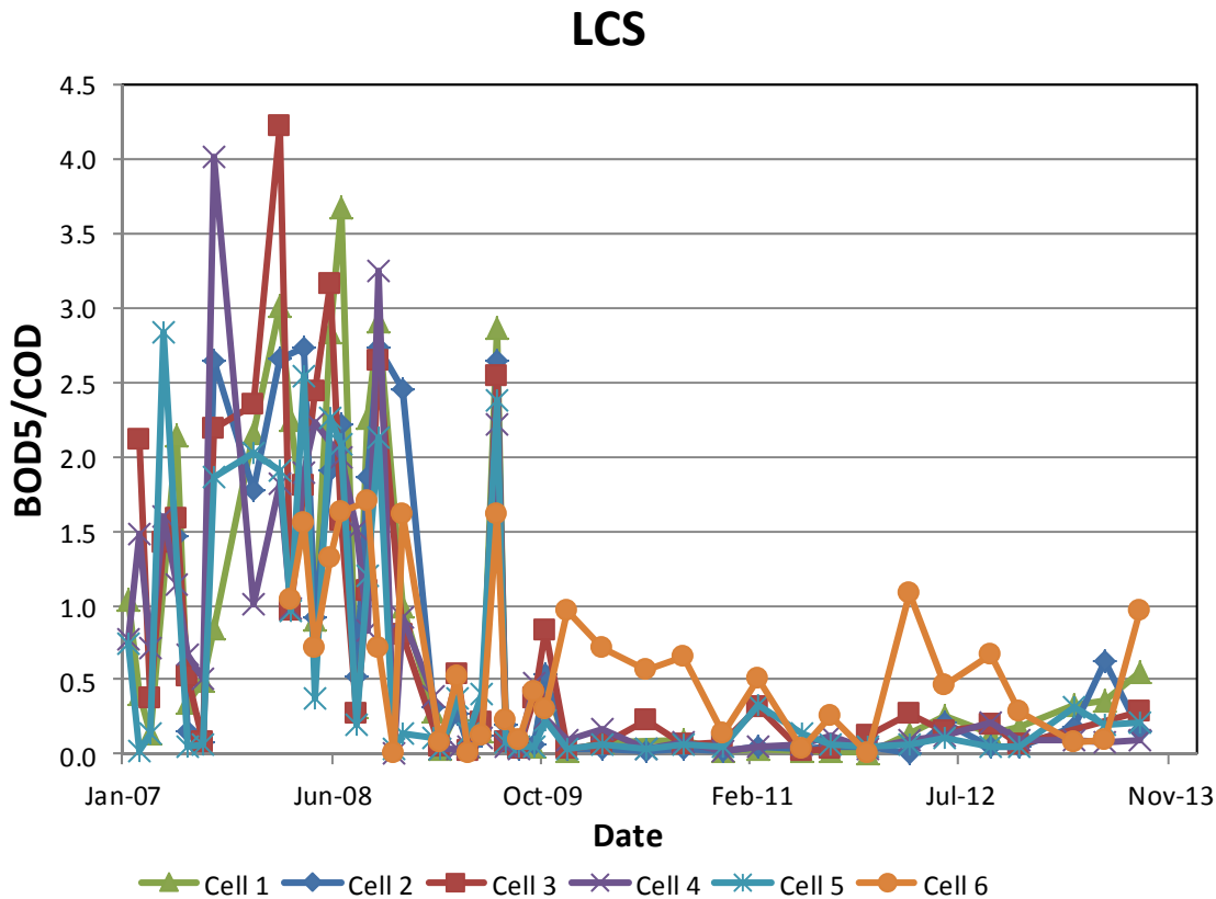
Figure 5-7 BOD5/COD Ratio of LCS in Cells 1-6
