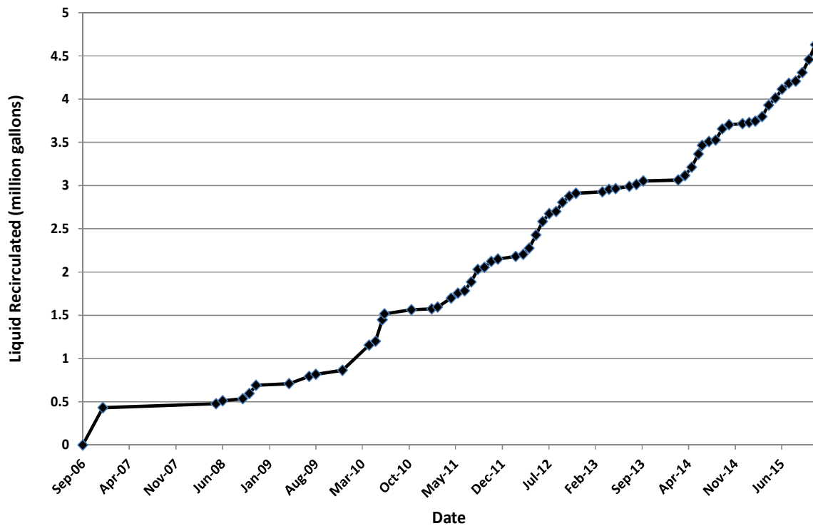
Figure 4-16 Cumulative Volume of Leachate Recirculated
