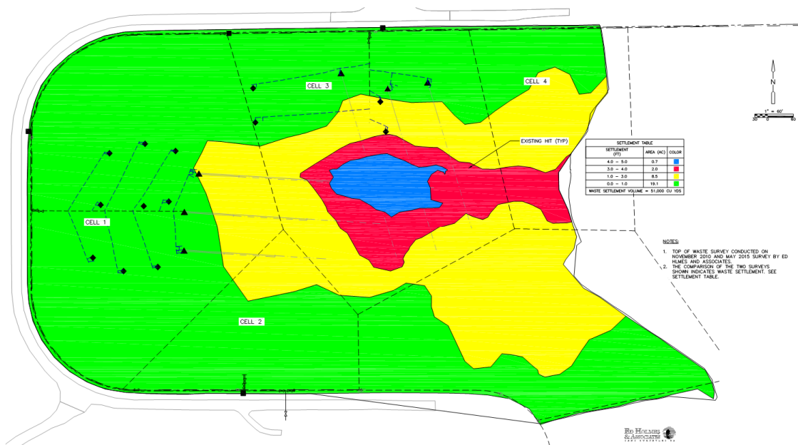
Figure ES-2: Settlement in Cells 1 through 5 since November 2010
