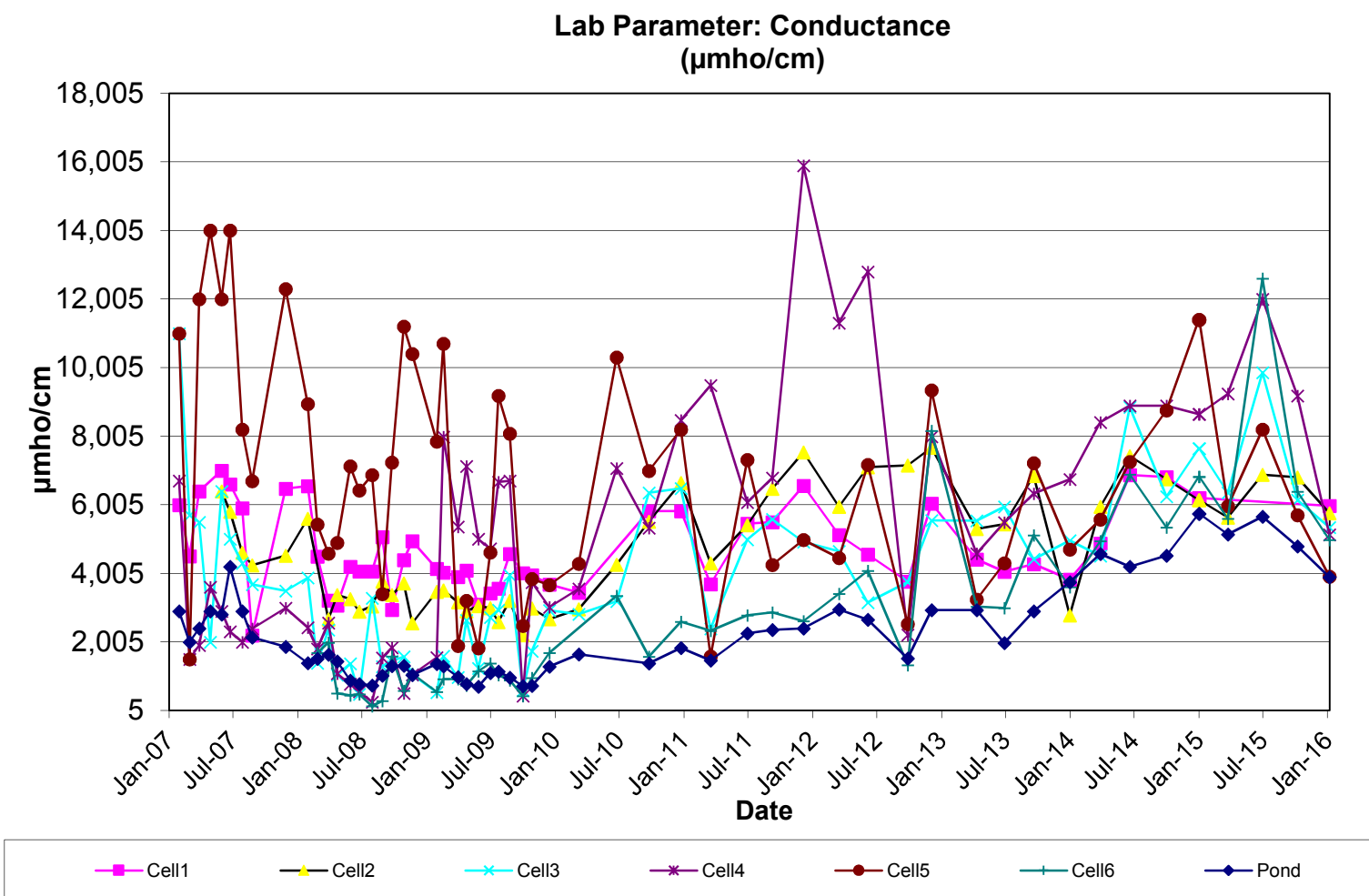
Figure 4-10 Specific Conductance of Leachate
