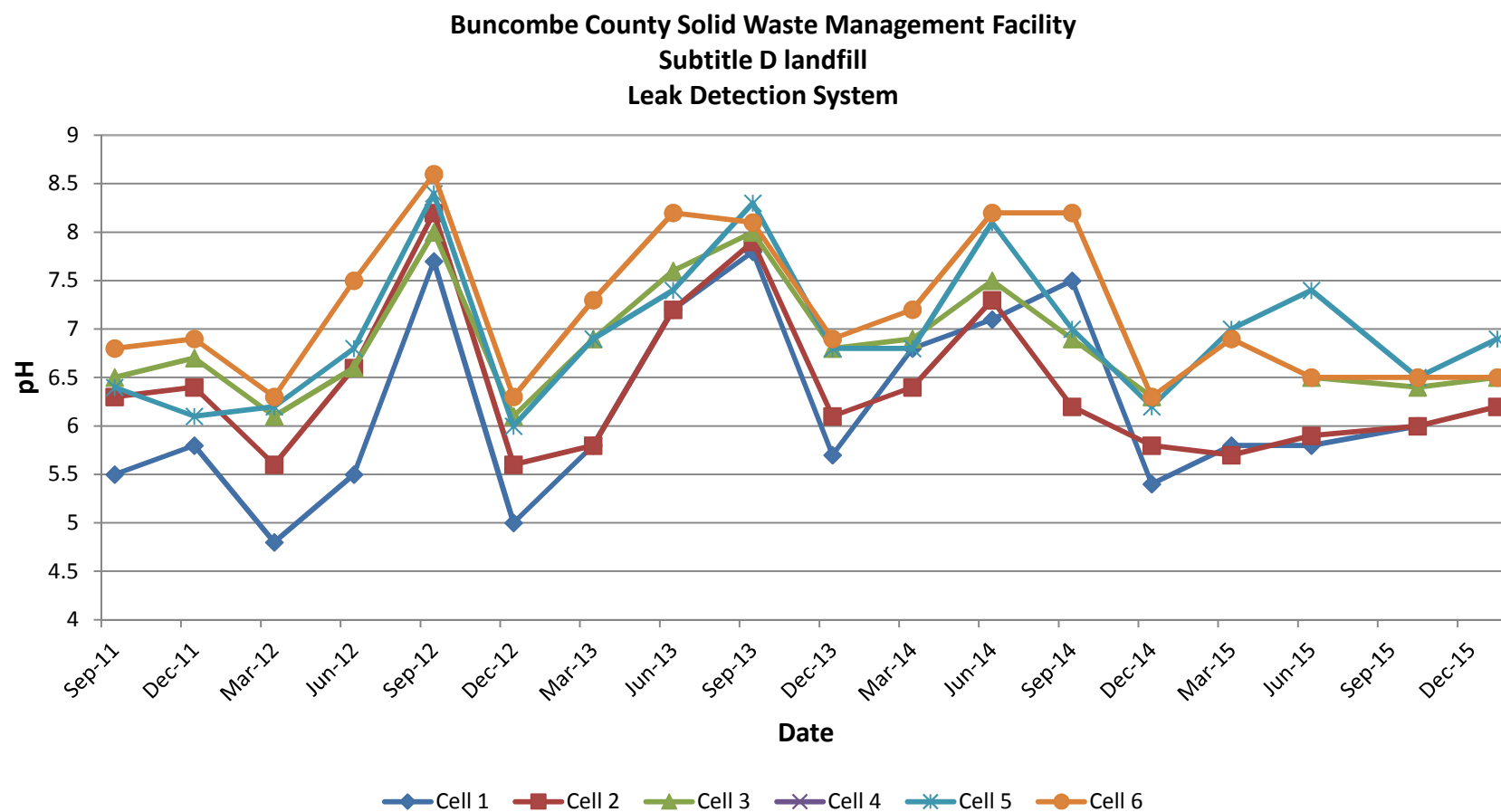
Figure 4-2 pH
