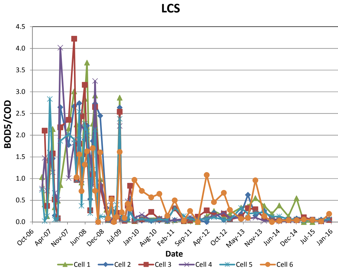
Figure 5-7 BOD5/COD Ratio of LCS in Cells 1-6
