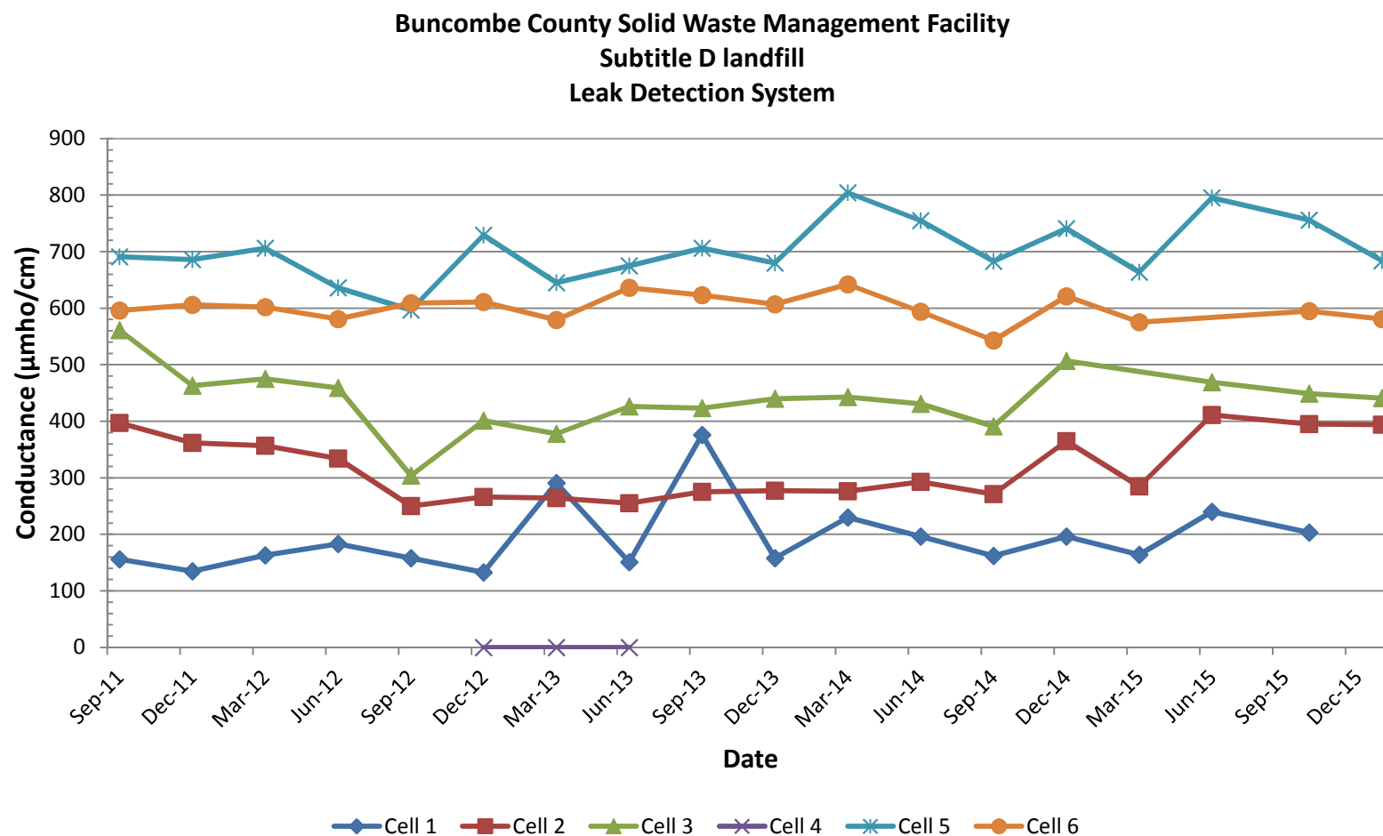
Figure 4-3 Specific Conductance
