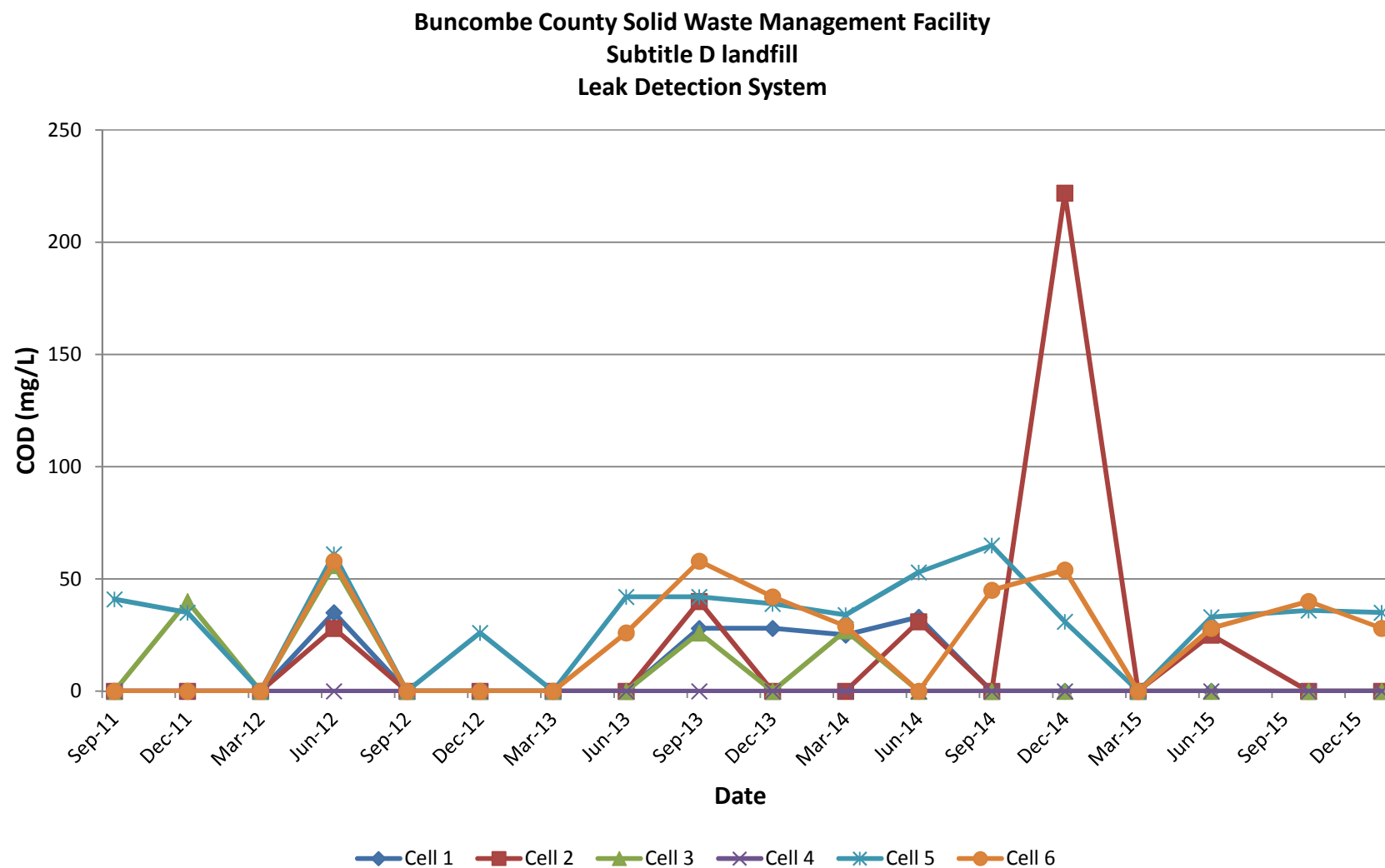
Figure 4-6 COD
