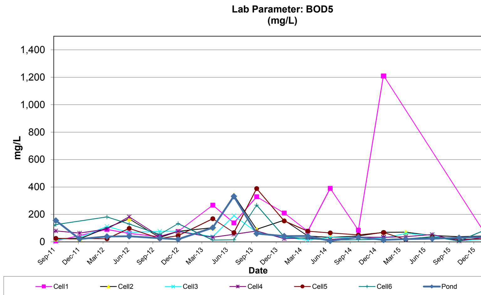
Figure 4-9 BOD5 of Leachate
