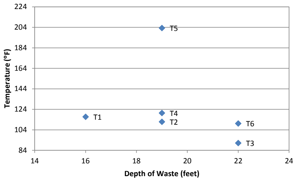
Figure 4-23 Temperature of Waste at Various Depths in Cell 6 (Note: Waste Depths from February 11, 2016 Topographic Survey and Temperature Reading from December 30, 2015)
