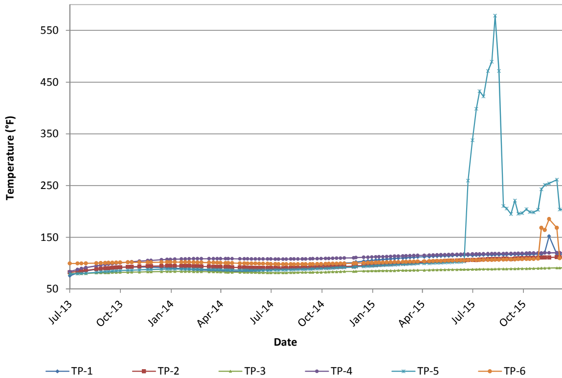
Figure 4-22 Waste Temperature Readings in Cell 6
