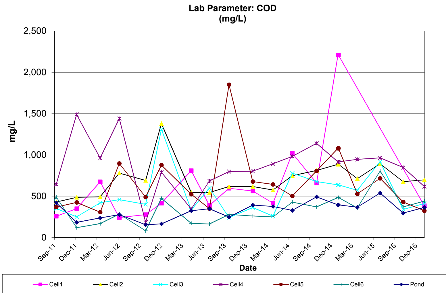
Figure 4-11 COD of Leachate
