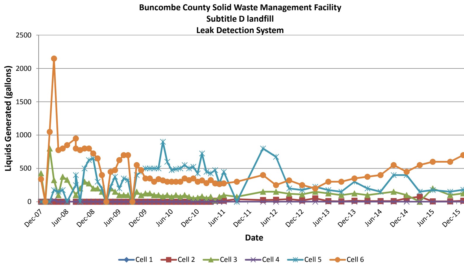
Figure 4-1 Quarterly Leak Detection Volumes
