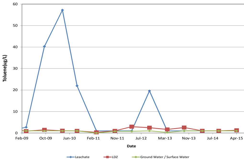
Figure 5-3 Toluene of Leachate, LDZ and GW/SW Samples (Values are averages of testing results for the six cells and all GW/SW monitoring wells)
