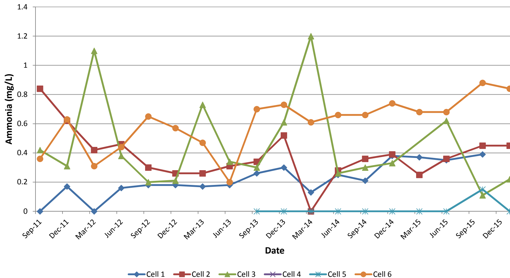
Figure 4-7 Ammonia
