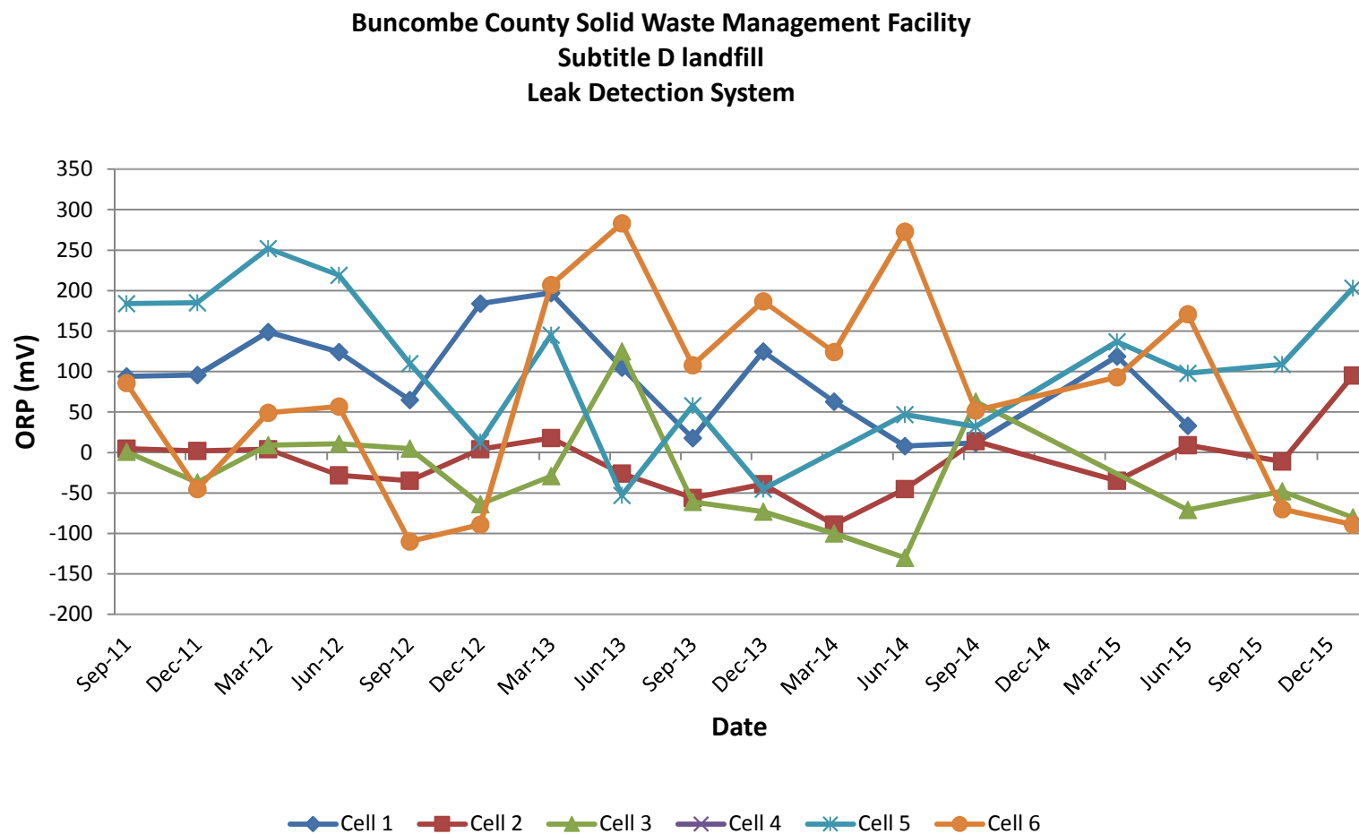
Figure 4-4 Oxidation Reduction Potential
