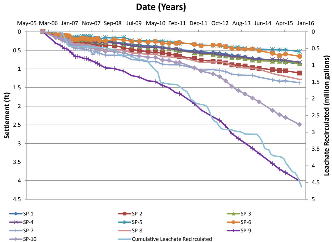
Figure 4-19 Cumulative Settlement
