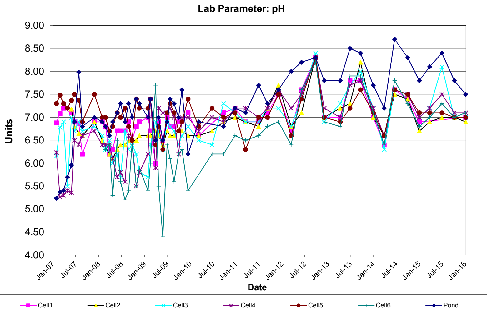
Figure 4-13 pH of Leachate
