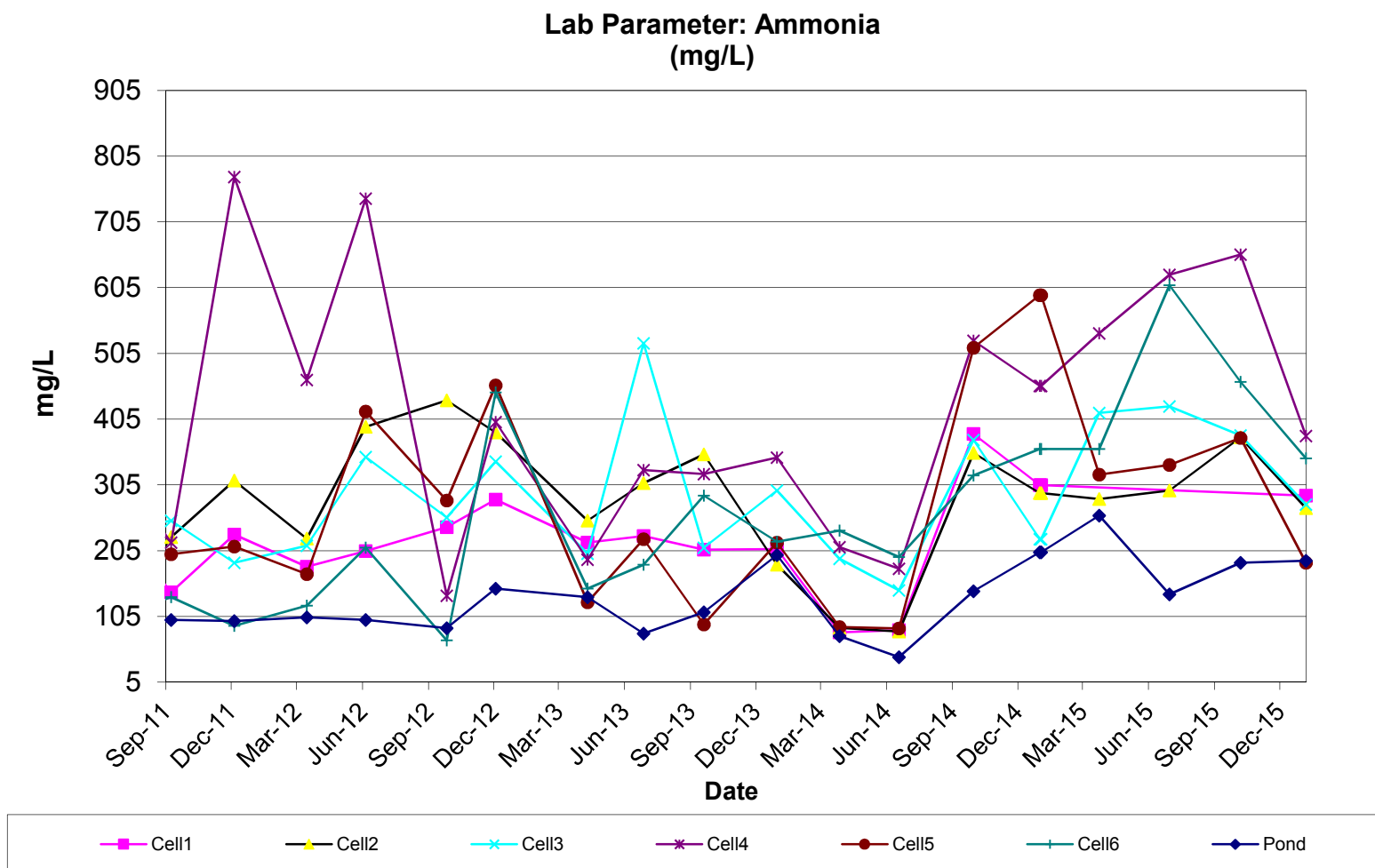
Figure 4-12 Ammonia of Leachate
