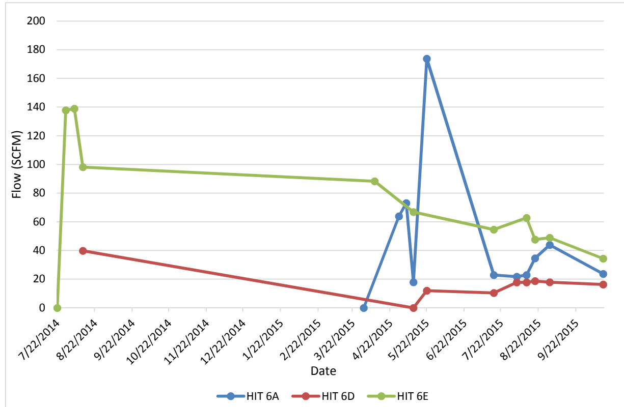
Figure 4-25 Flow Rate in HITs 6A, 6D, and 6E
