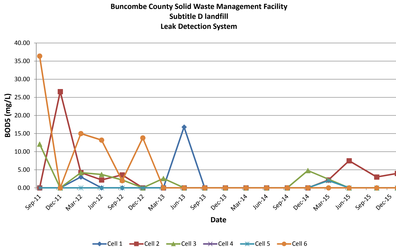
Figure 4-5 BOD5
