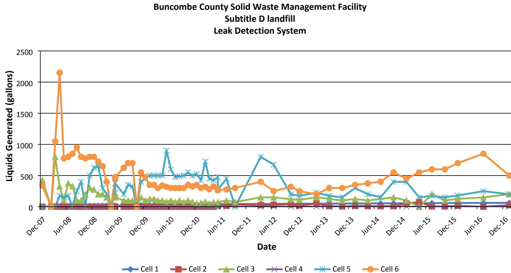
Figure 4-1 Semi-Annual Leak Detection Volumes
