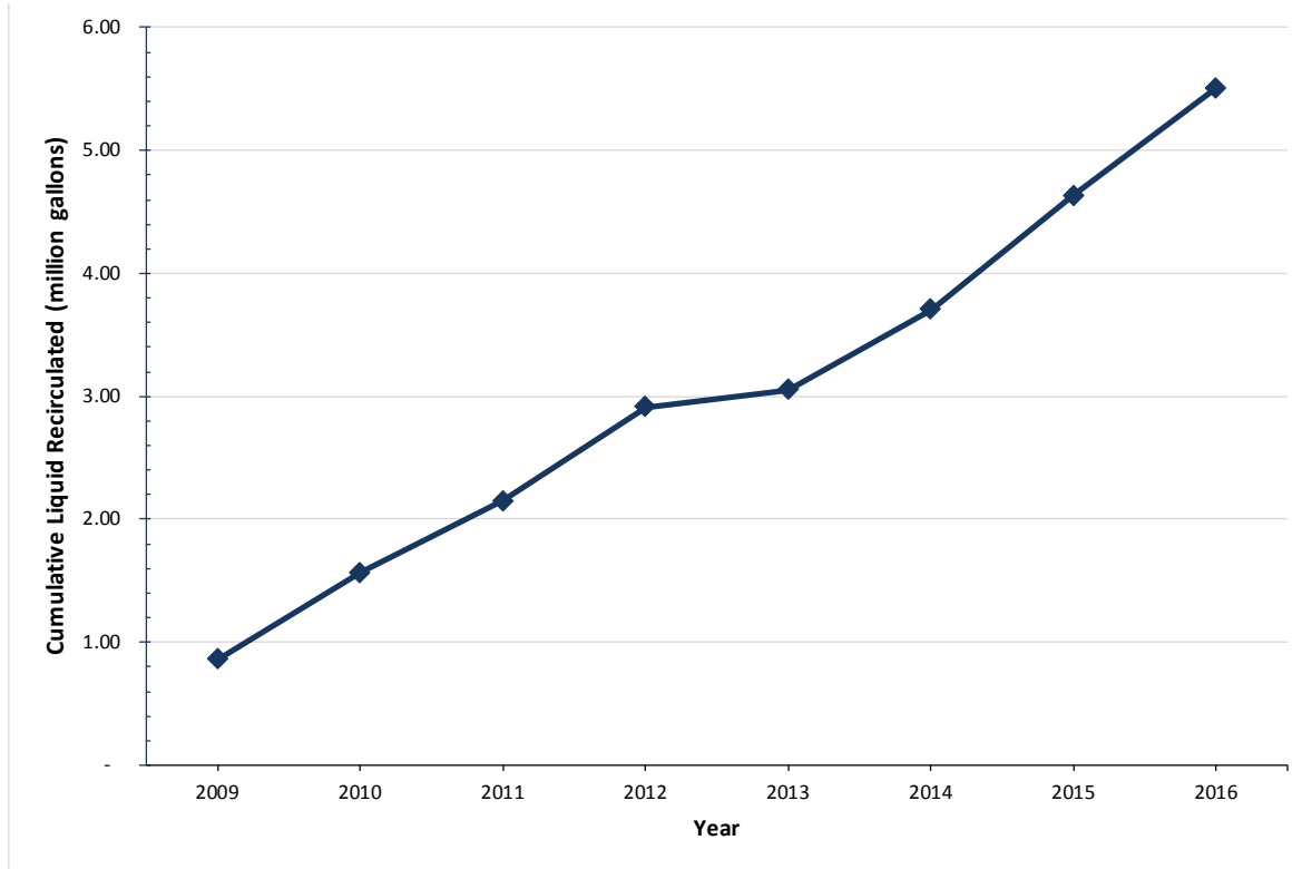
Figure 4-16 Cumulative Volume of Leachate Recirculated
