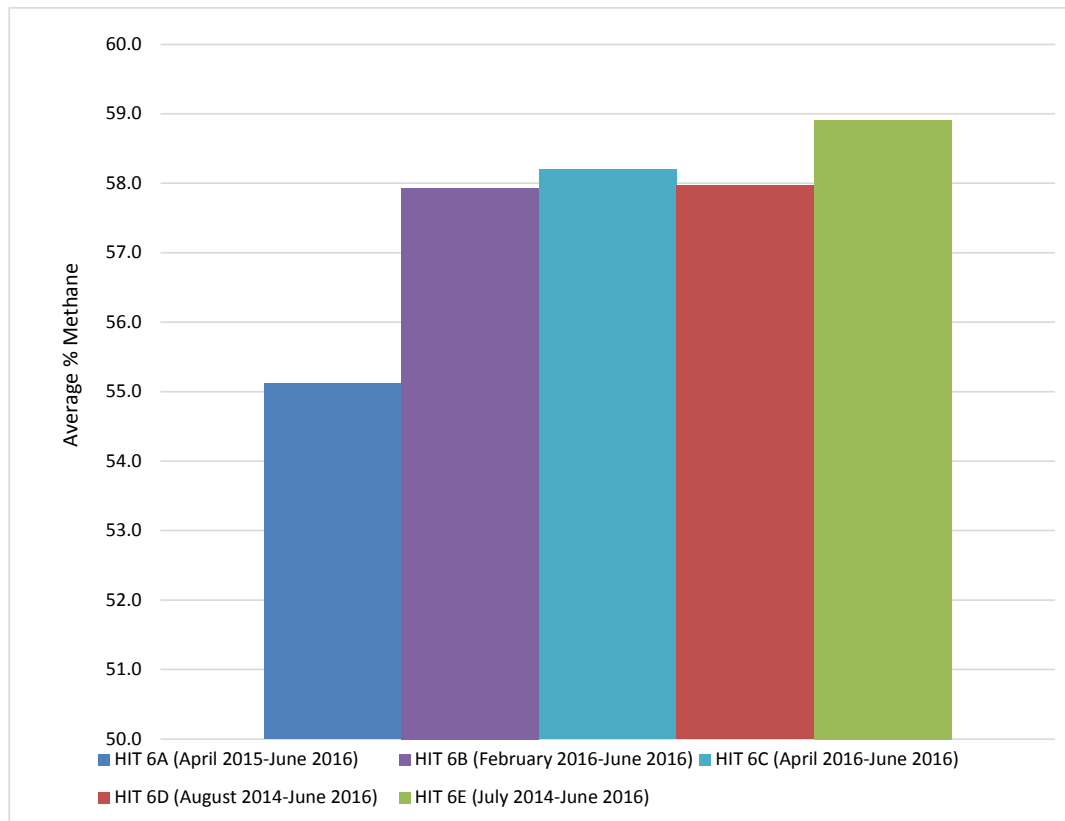
Figure 4-24 Average Percent Methane in HITs 6A, 6B, 6C, 6D, and 6E
