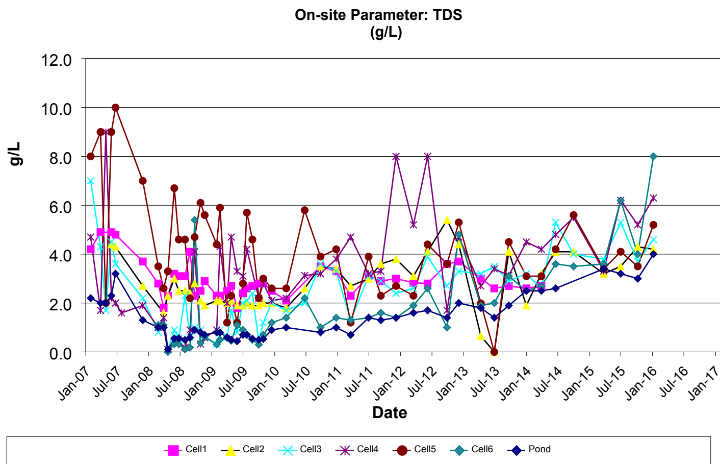
Figure 4-15 TDS of Leachate
