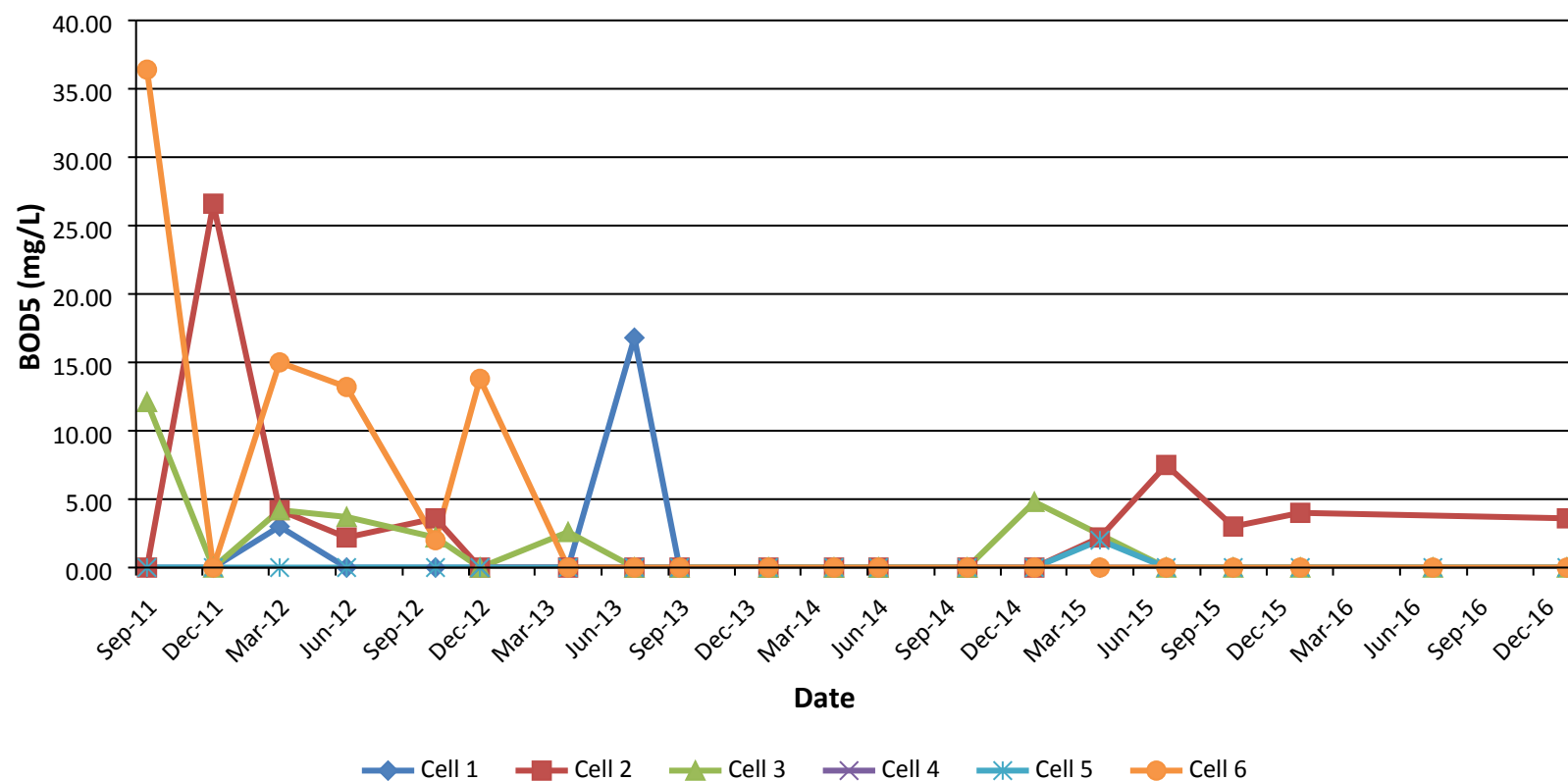
Figure 4-5 BOD5
