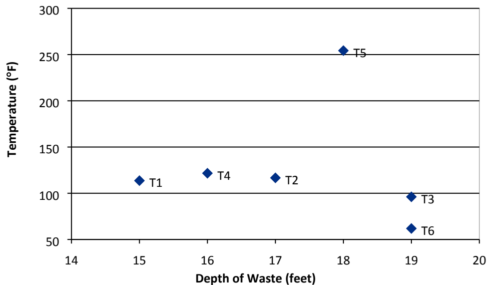
Figure 4-23 Temperature of Waste at Various Depths in Cell 6
