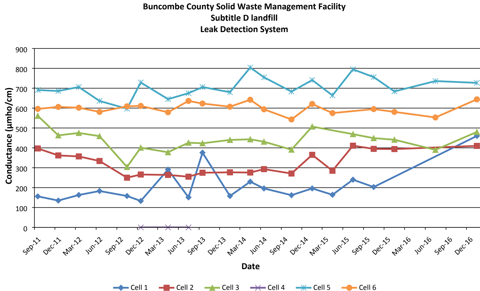
Figure 4-3 Specific Conductance
