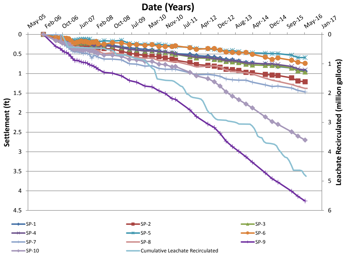
Figure 4-19 Cumulative Settlement
