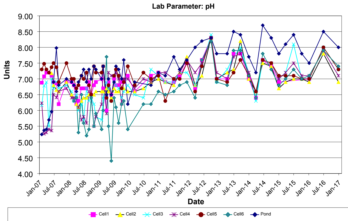
Figure 4-13 pH of Leachate
