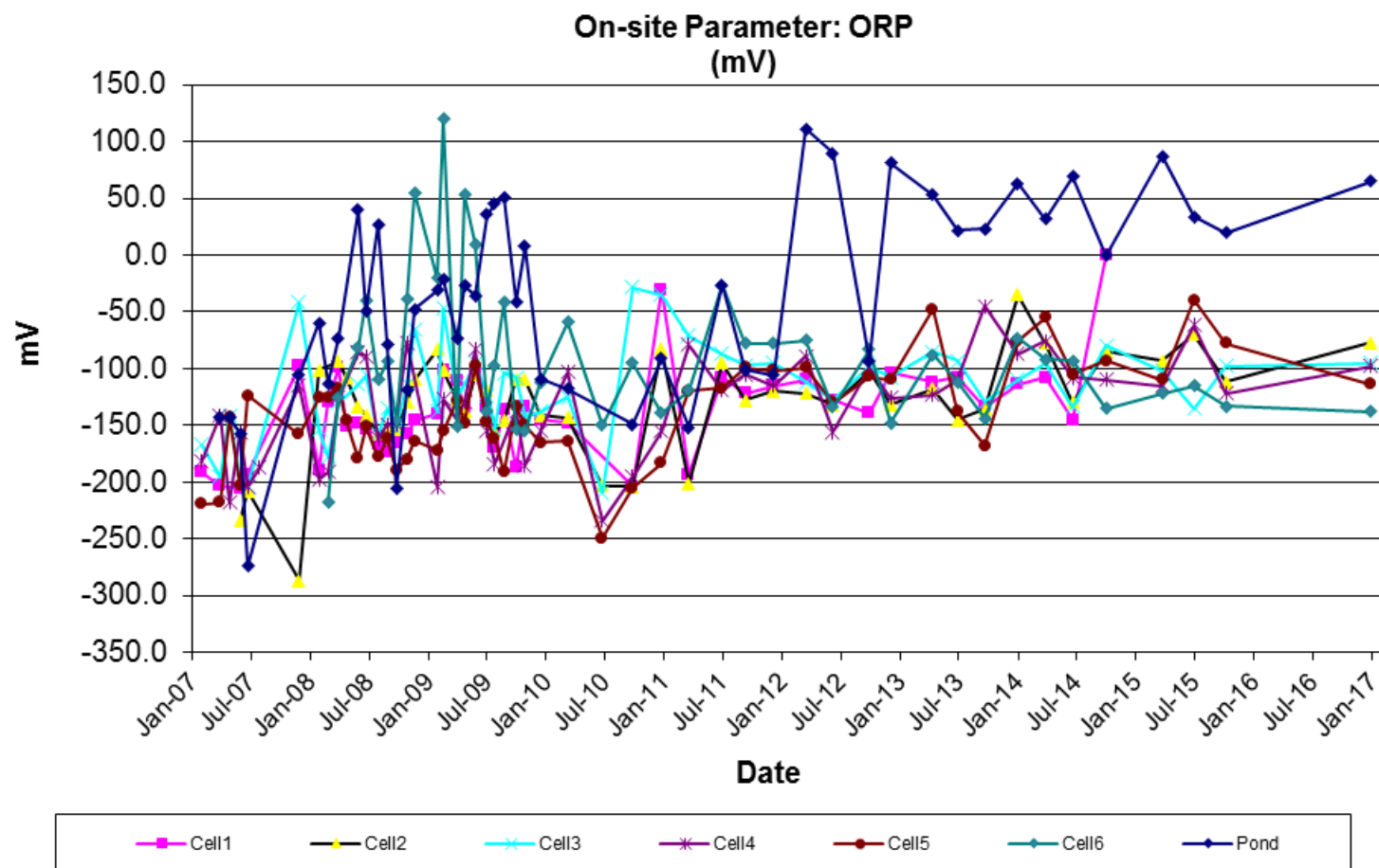
Figure 4-14 ORP of Leachate
