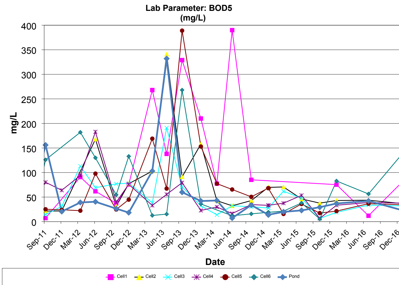
Figure 4-9 BOD5 of Leachate
