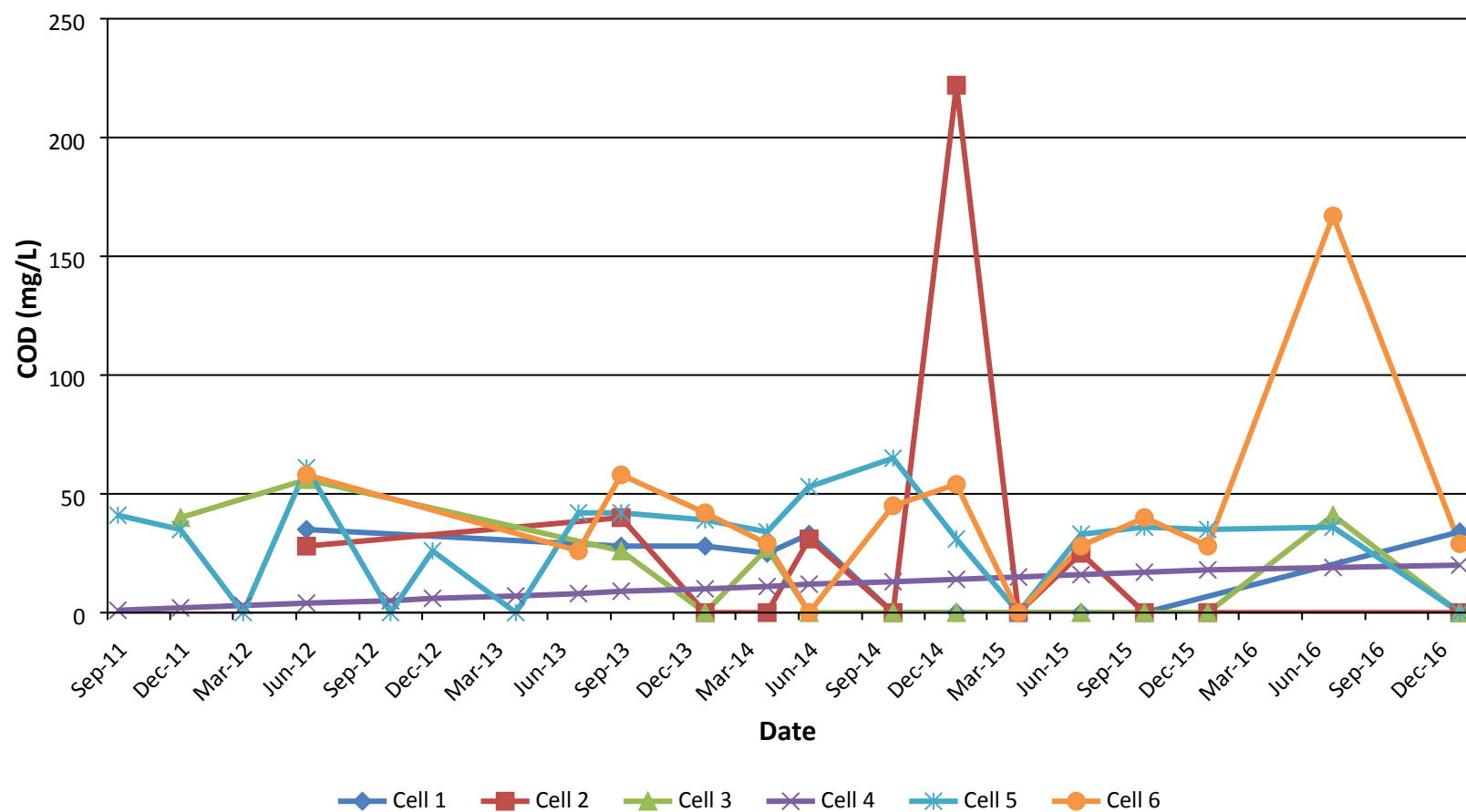
Figure 4-6 COD
