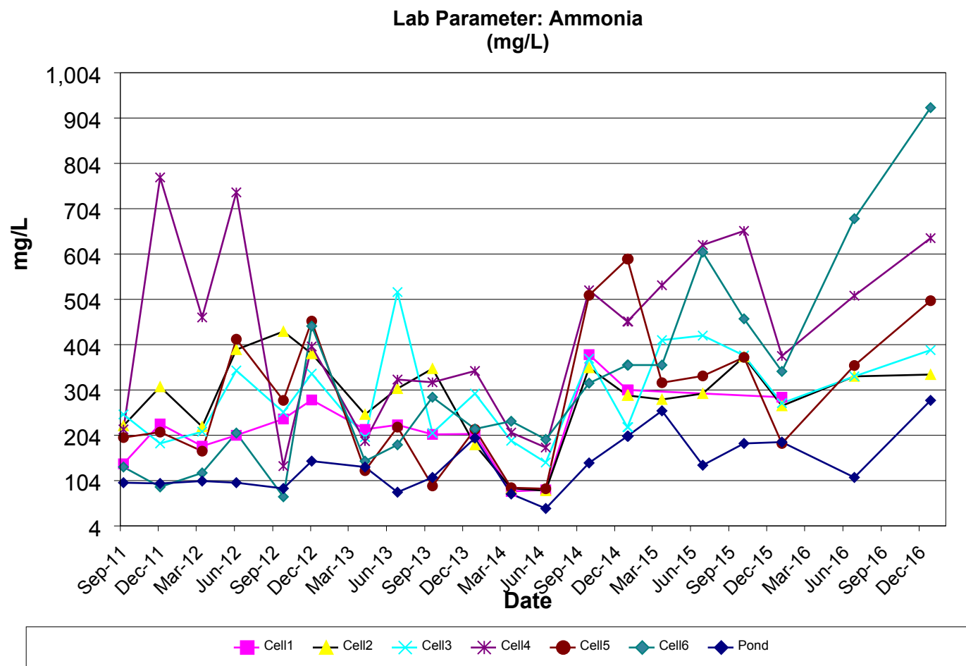
Figure 4-12 Ammonia of Leachate
