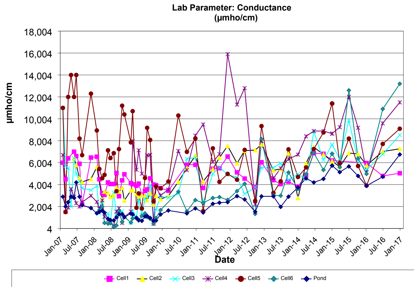
Figure 4-10 Specific Conductance of Leachate
