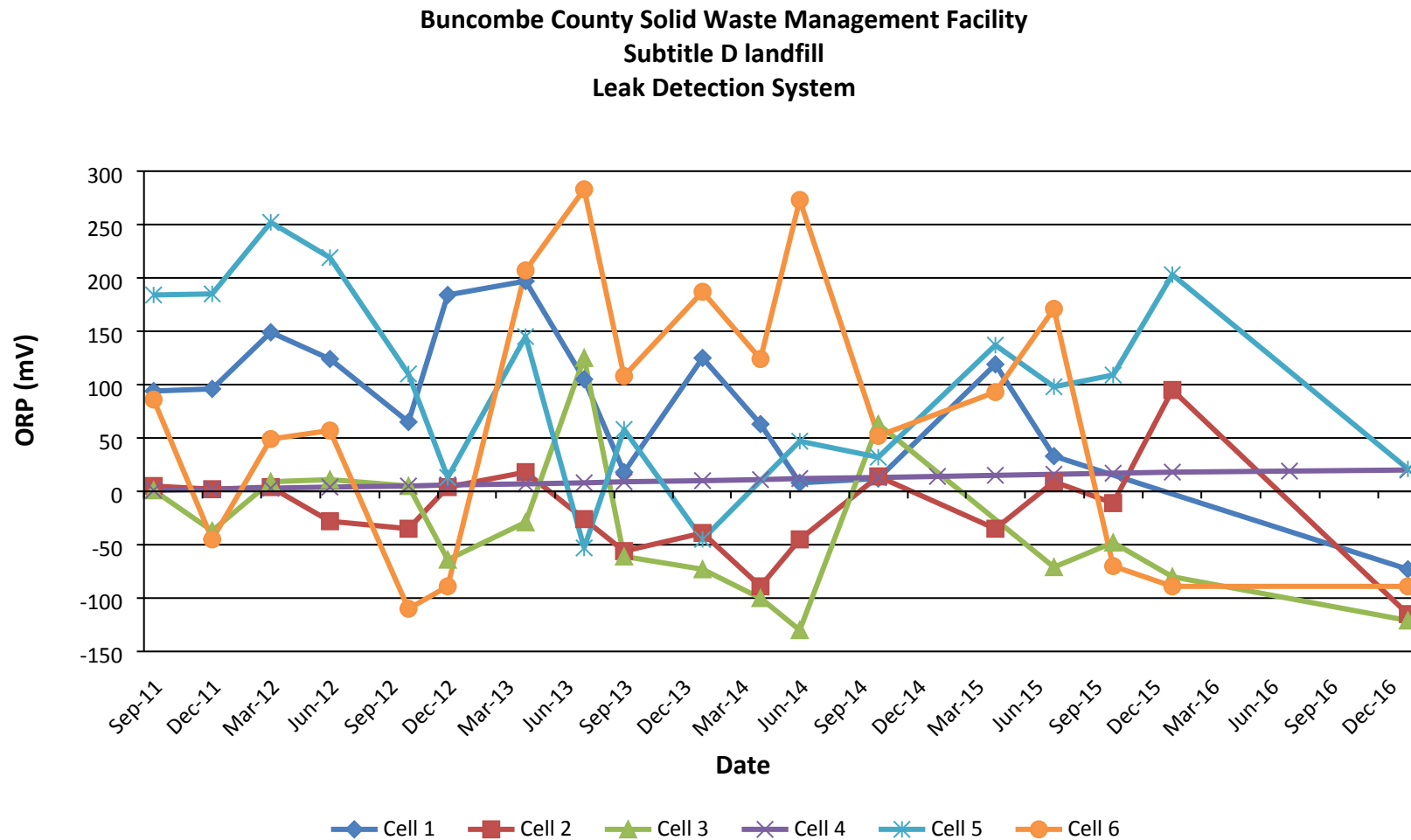
Figure 4-4 Oxidation Reduction Potential
