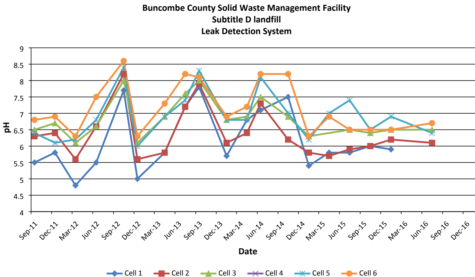
Figure 4-2 pH
