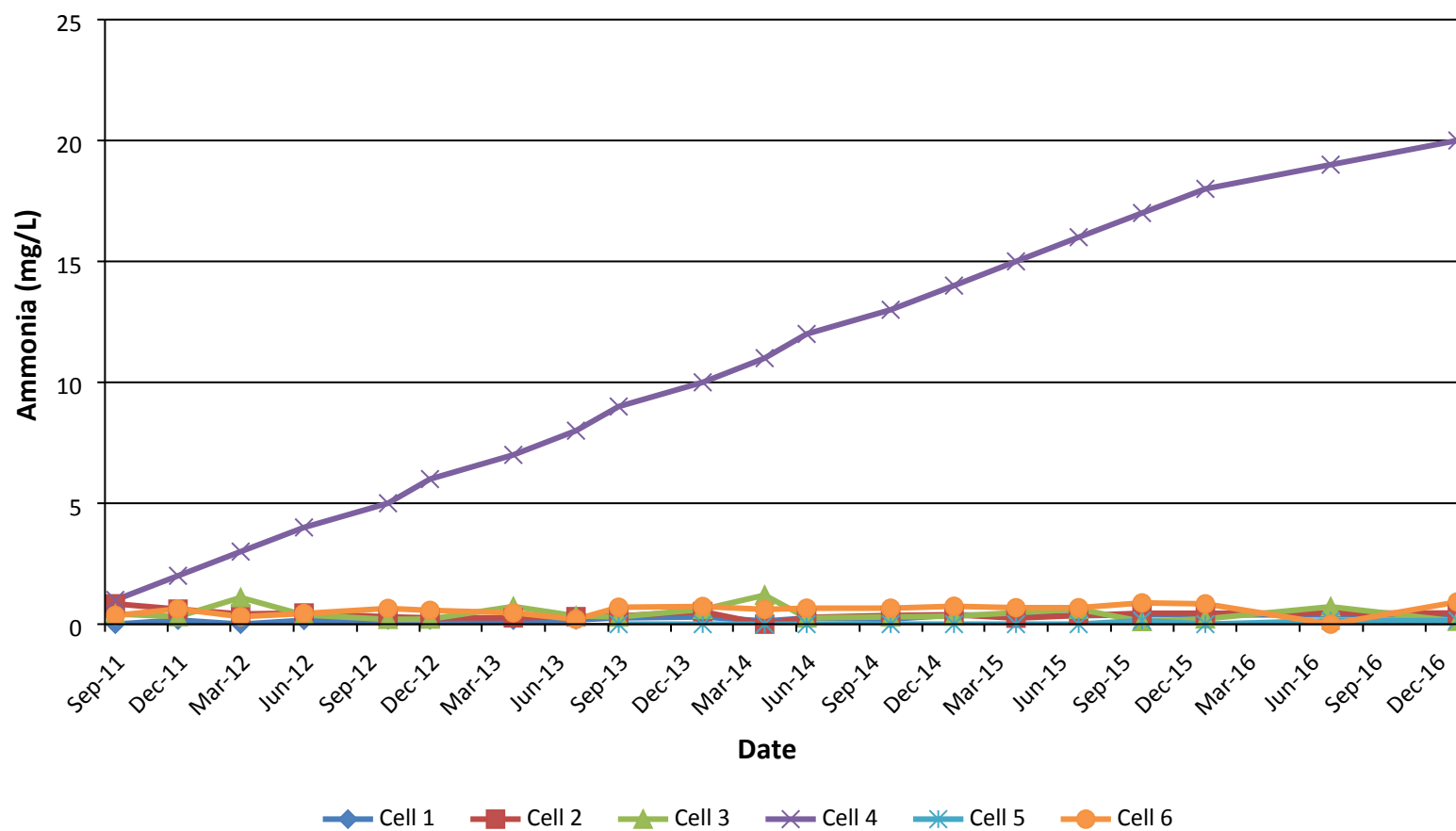
Figure 4-7 Ammonia
