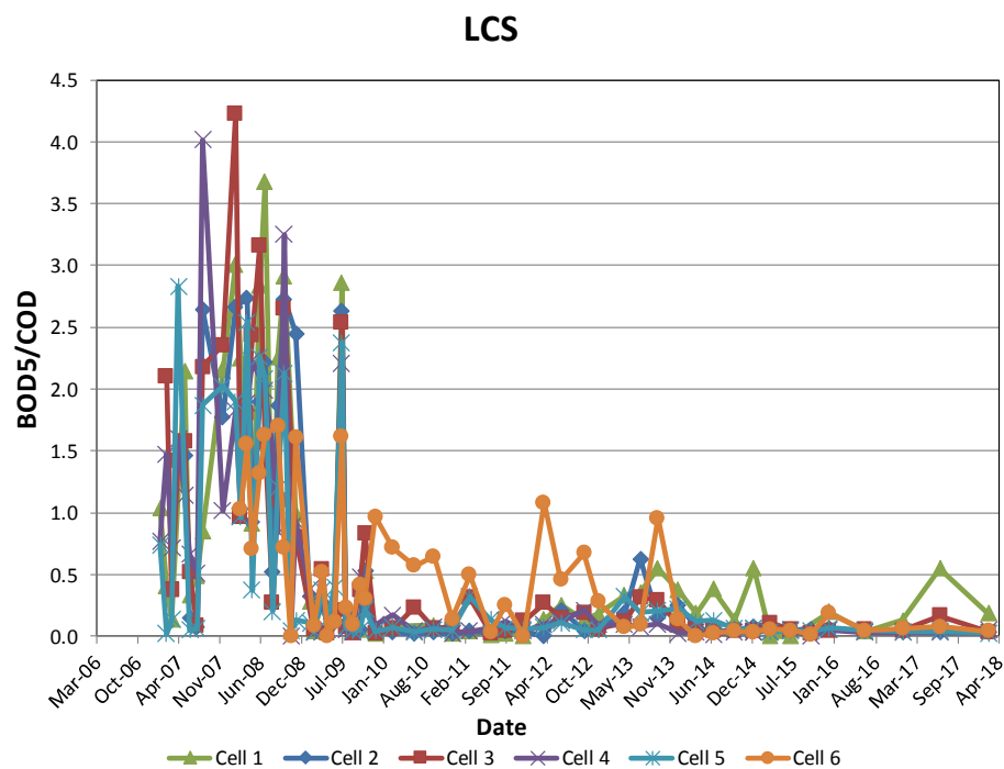
Figure 5-7 BOD 5 /COD Ratio of LCS in Cells 1-6
