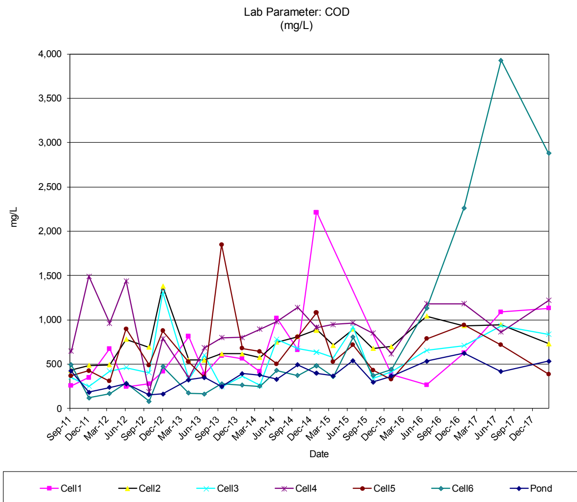
Figure 4-11 COD of Leachate
