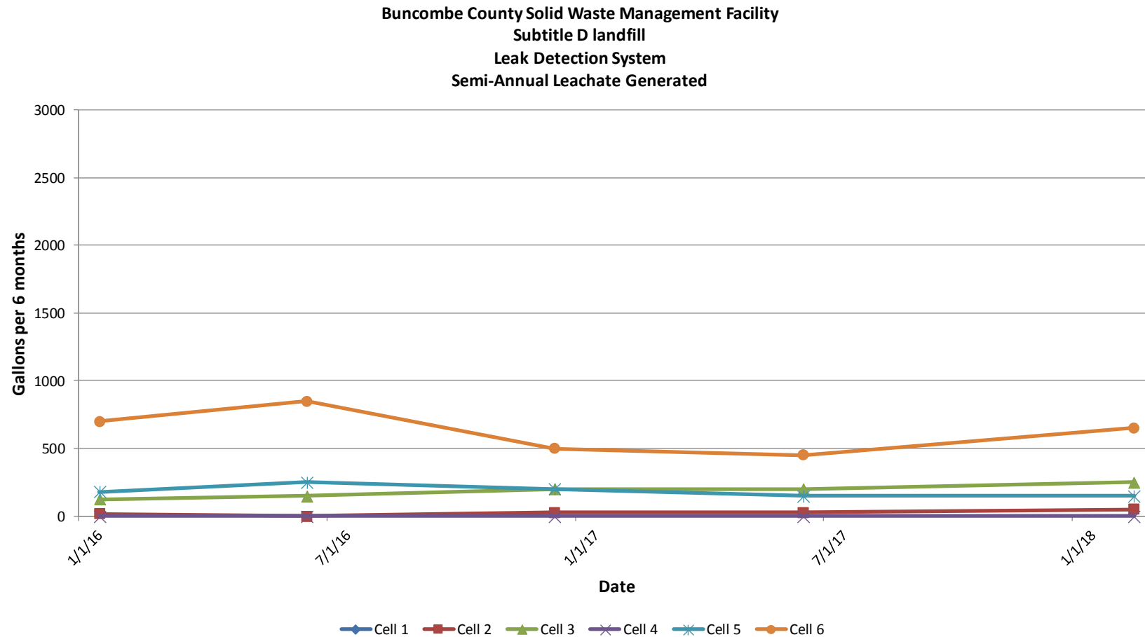
Figure 4-1b Semi-Annual Leak Detection Volumes (2016-present)
