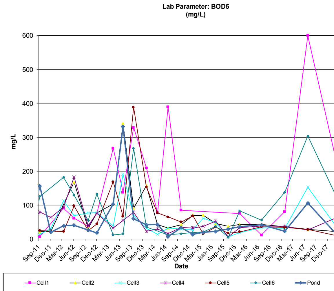
Figure 4-9 BOD5 of Leachate
