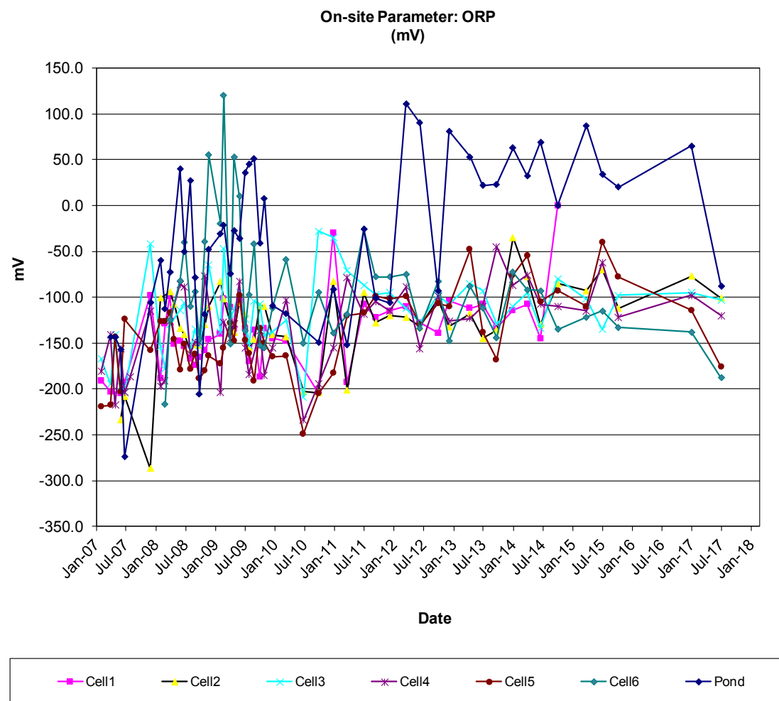
Figure 4-14 ORP of Leachate
