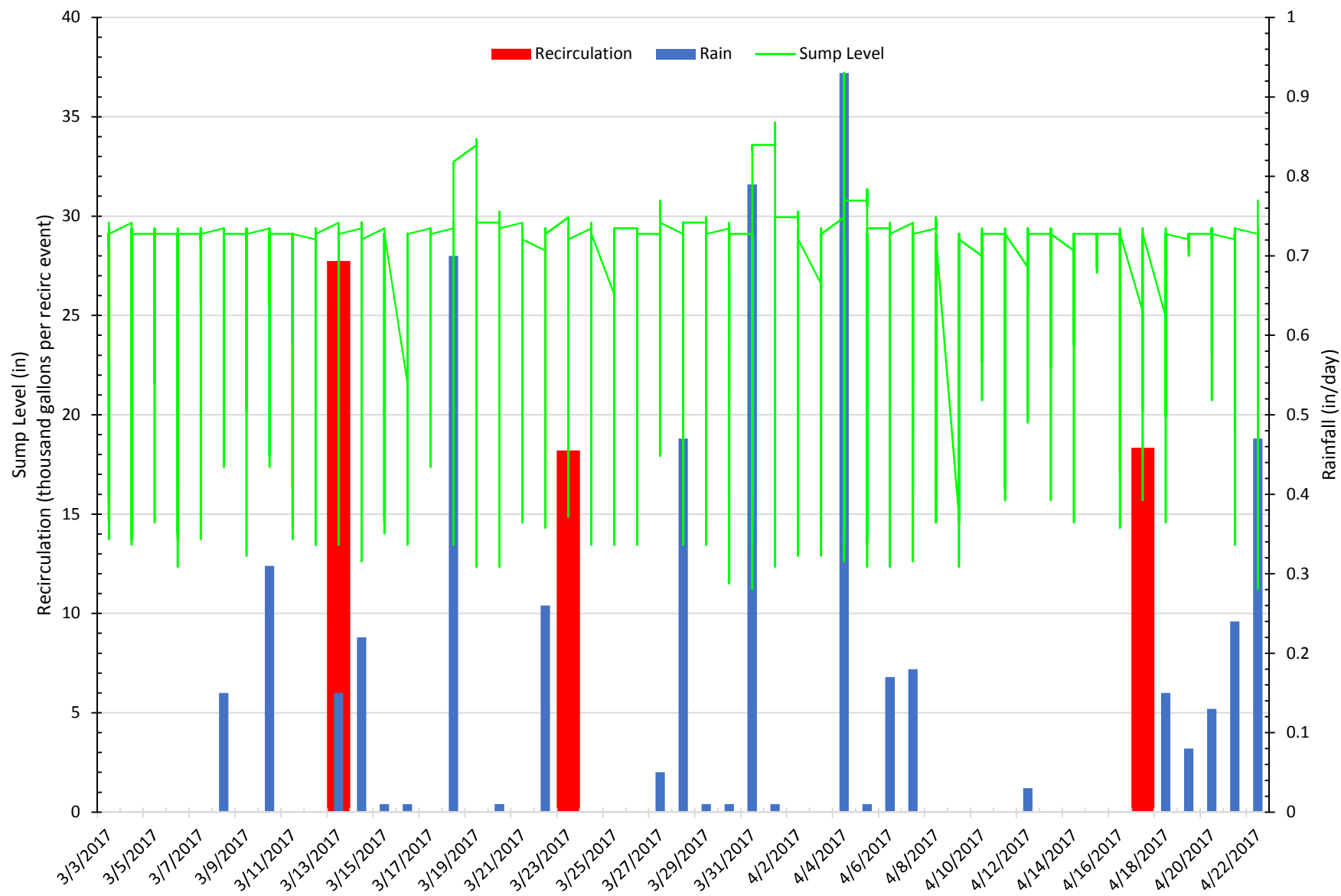
Figure 4-27 Cell 6 Sump Level, Cell 6 HITs Recirculation Events, and Rainfall (March-April 2017)
