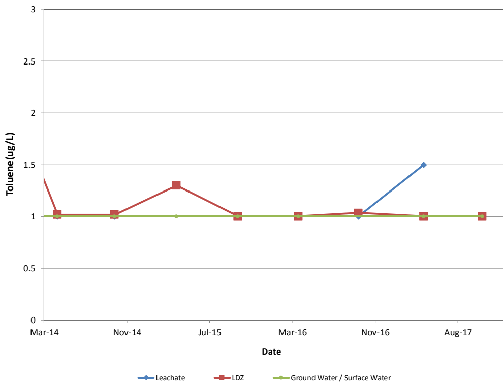
Figure 5-3 Toluene of Leachate, LDZ and GW/SW Samples (Values are averages of testing results for the six cells and all GW/SW monitoring wells)
