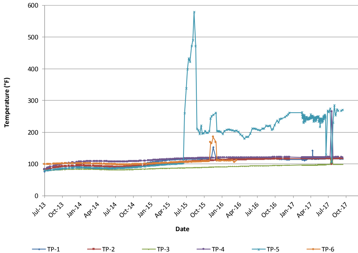
Figure 4-22 Waste Temperature Readings in Cell 6
