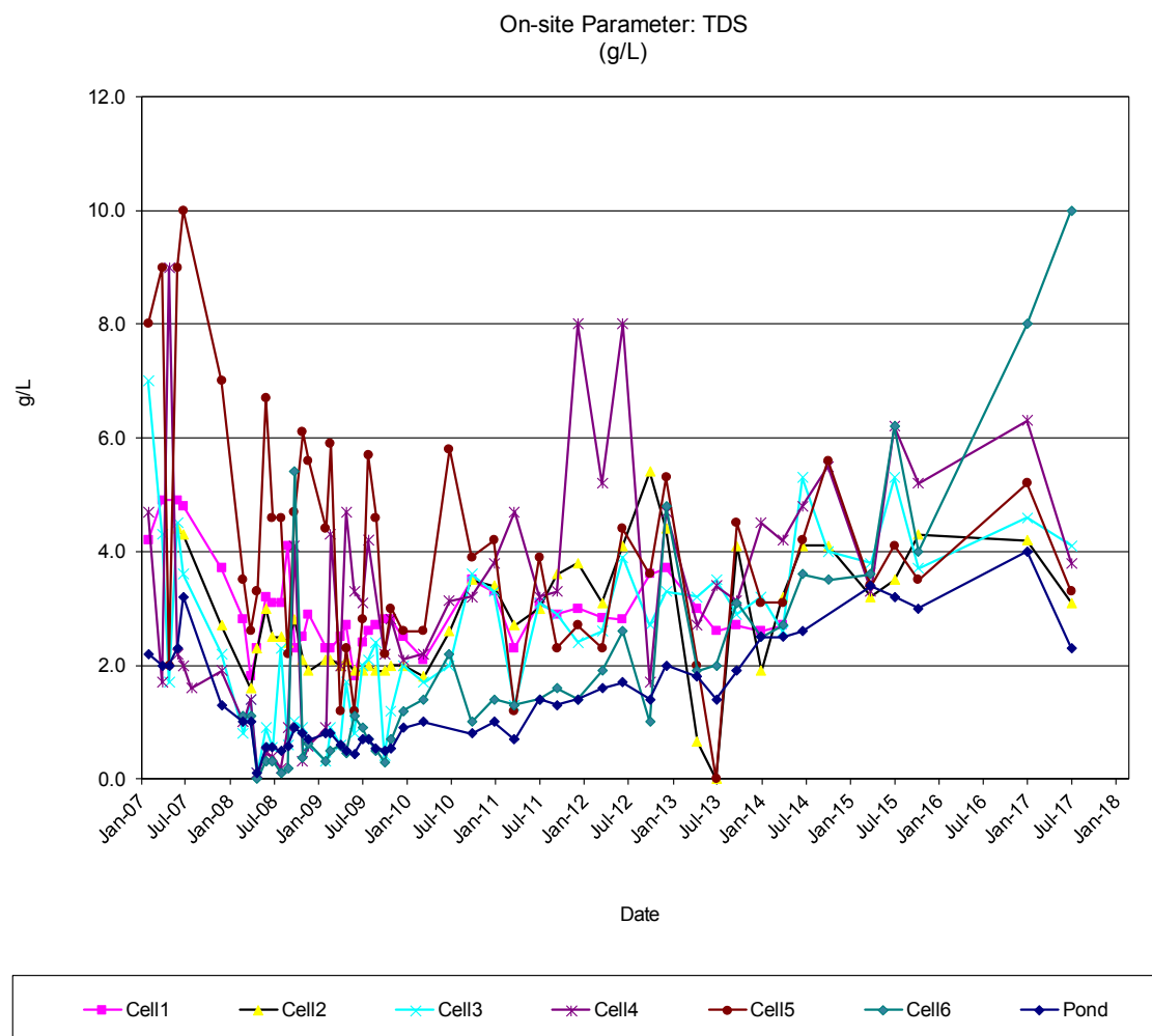
Figure 4-15 TDS of Leachate
