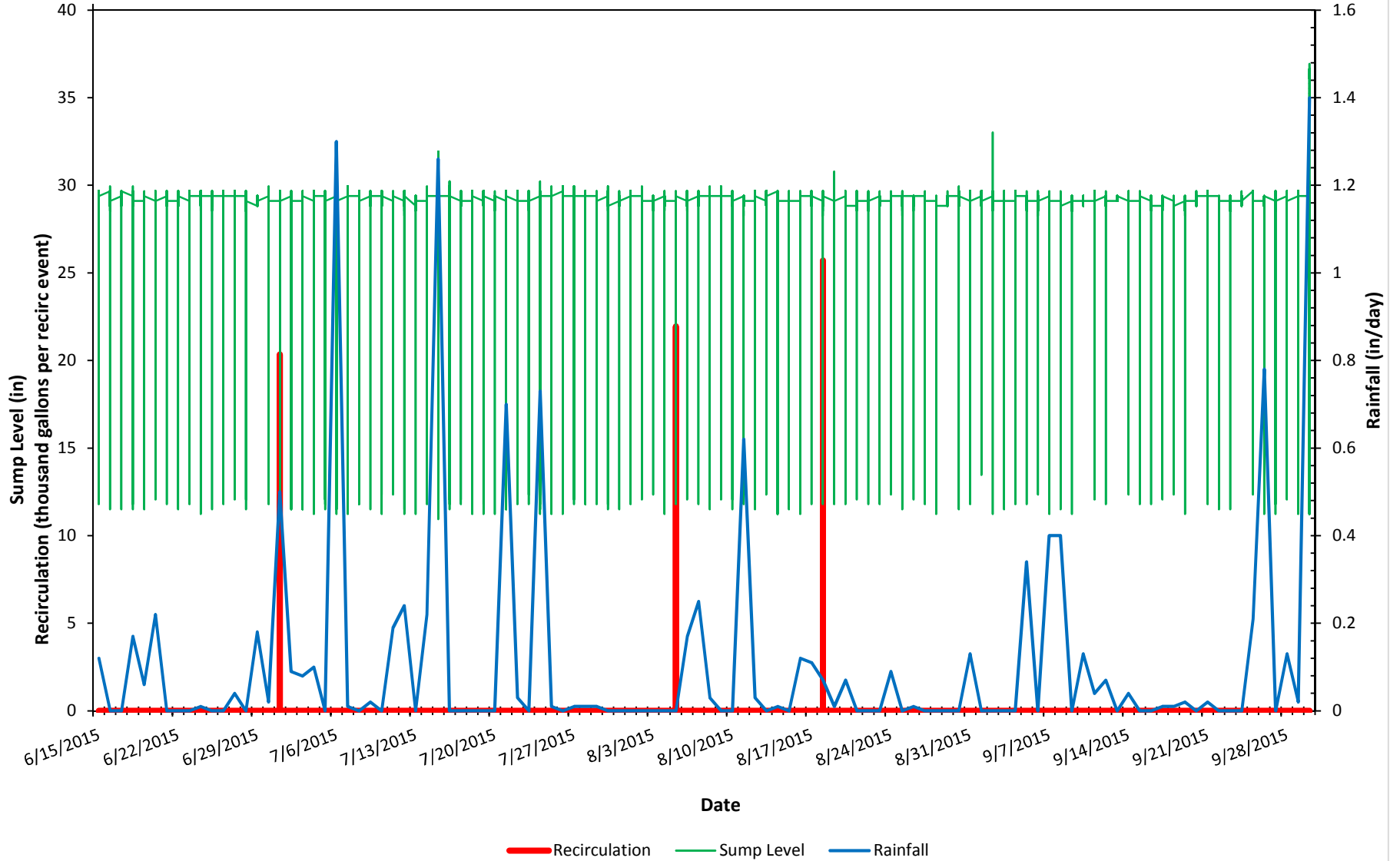
Figure 4-26 Cell 6 Sump Level, Cell 6 HITs Recirculation Events, and Rainfall
