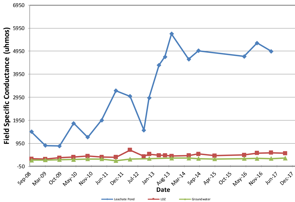
Figure 5-2 Conductance of Leachate, LDZ, and GW Samples (Values are averages of testing results for the six cells and all GW monitoring wells)
