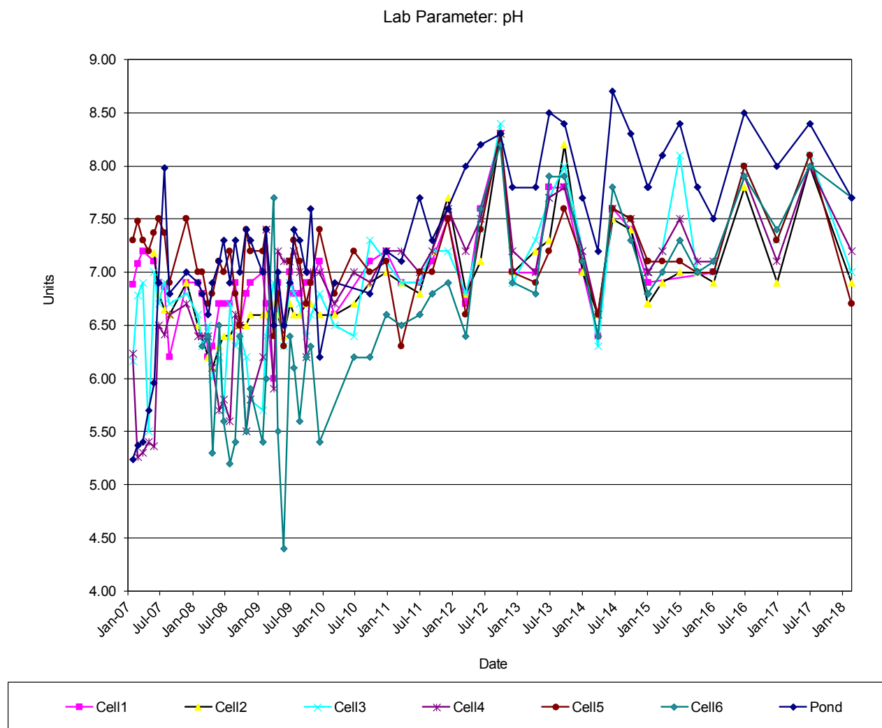
Figure 4-13 pH of Leachate
