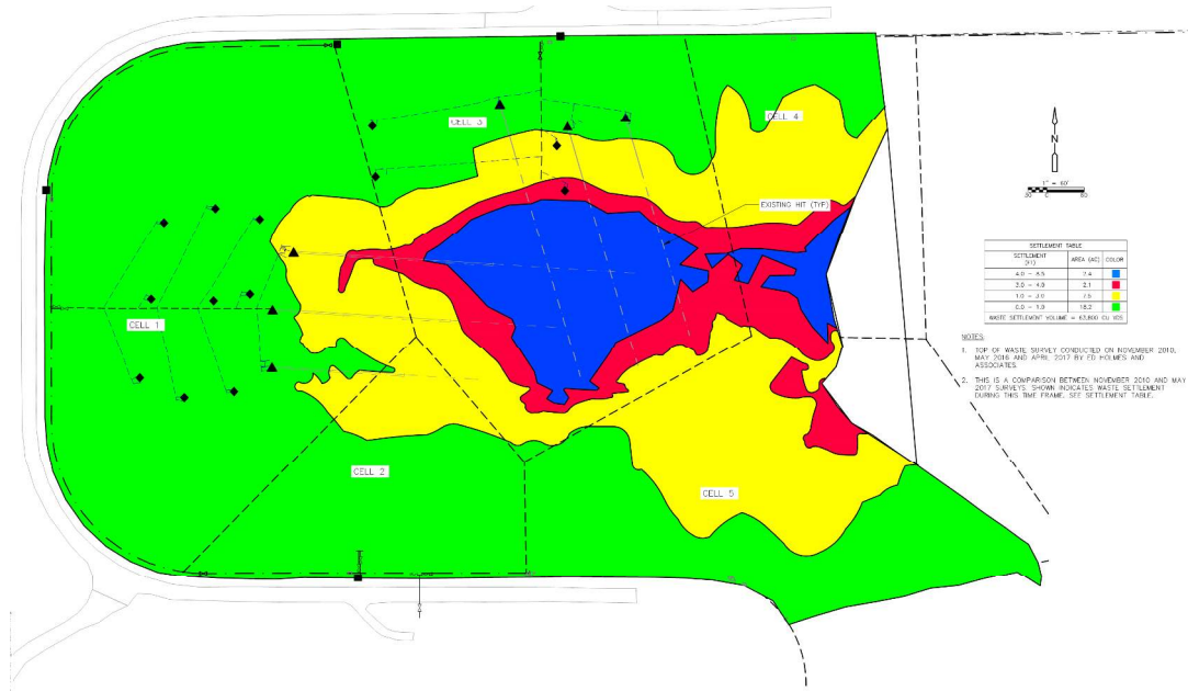
Figure ES-6: Settlement in Cells 1 through 5 since November 2010
