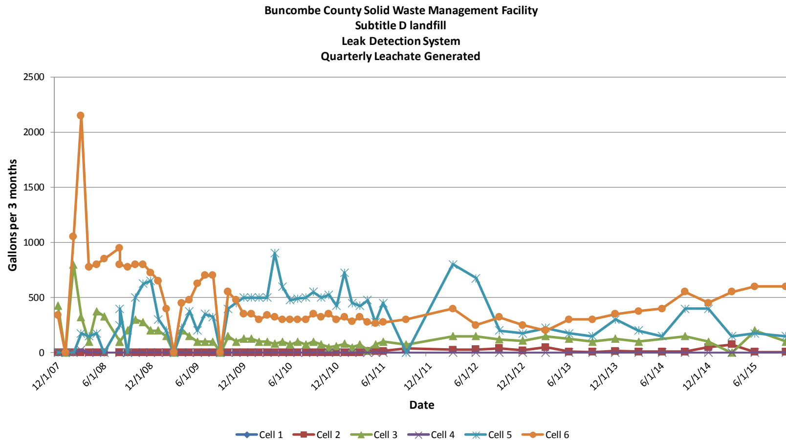
Figure 4-1a Quarterly Leak Detection Volumes (2007-2015)
