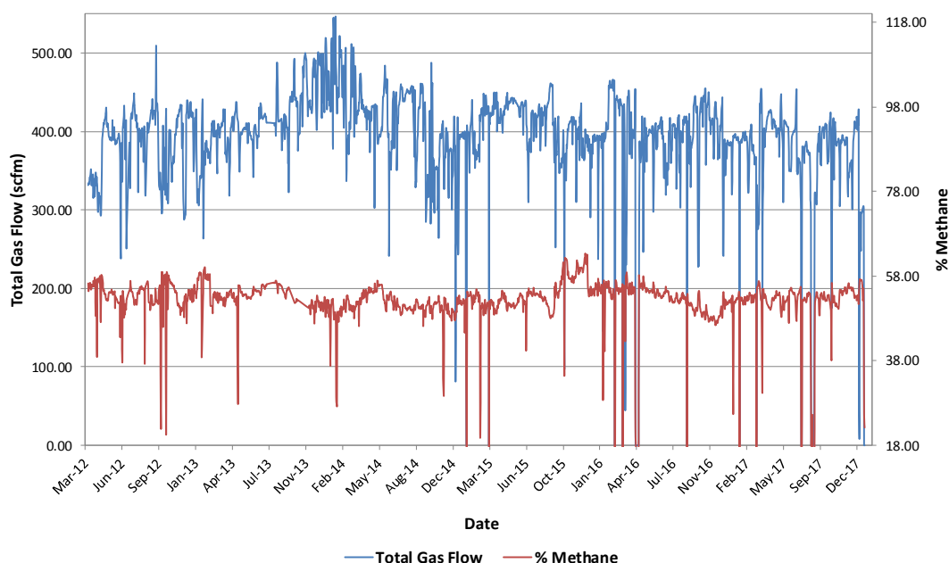
Figure 4-17 Total Gas Flow and Percent Methane at the LFGTE Facility
