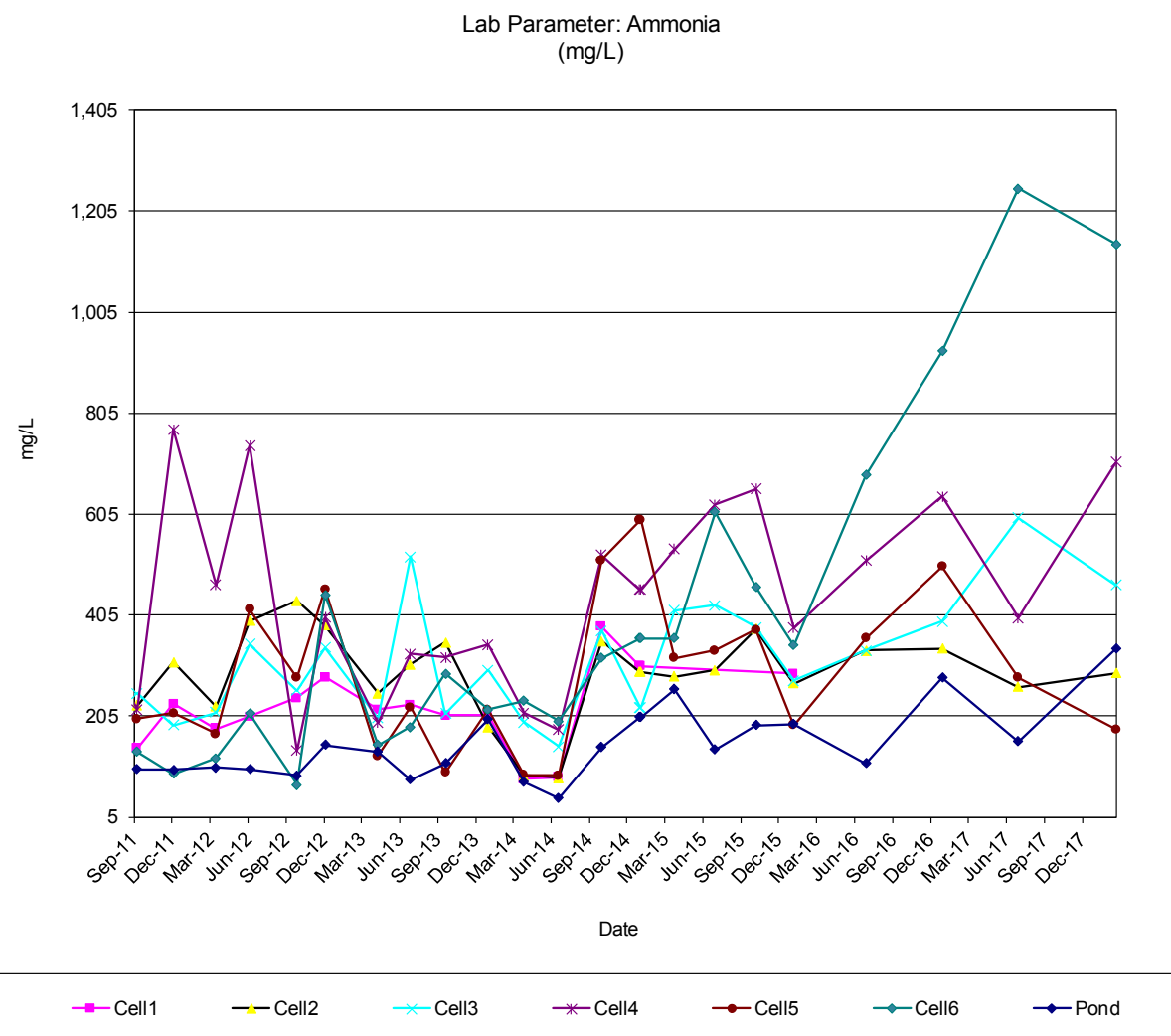
Figure 4-12 Ammonia of Leachate
