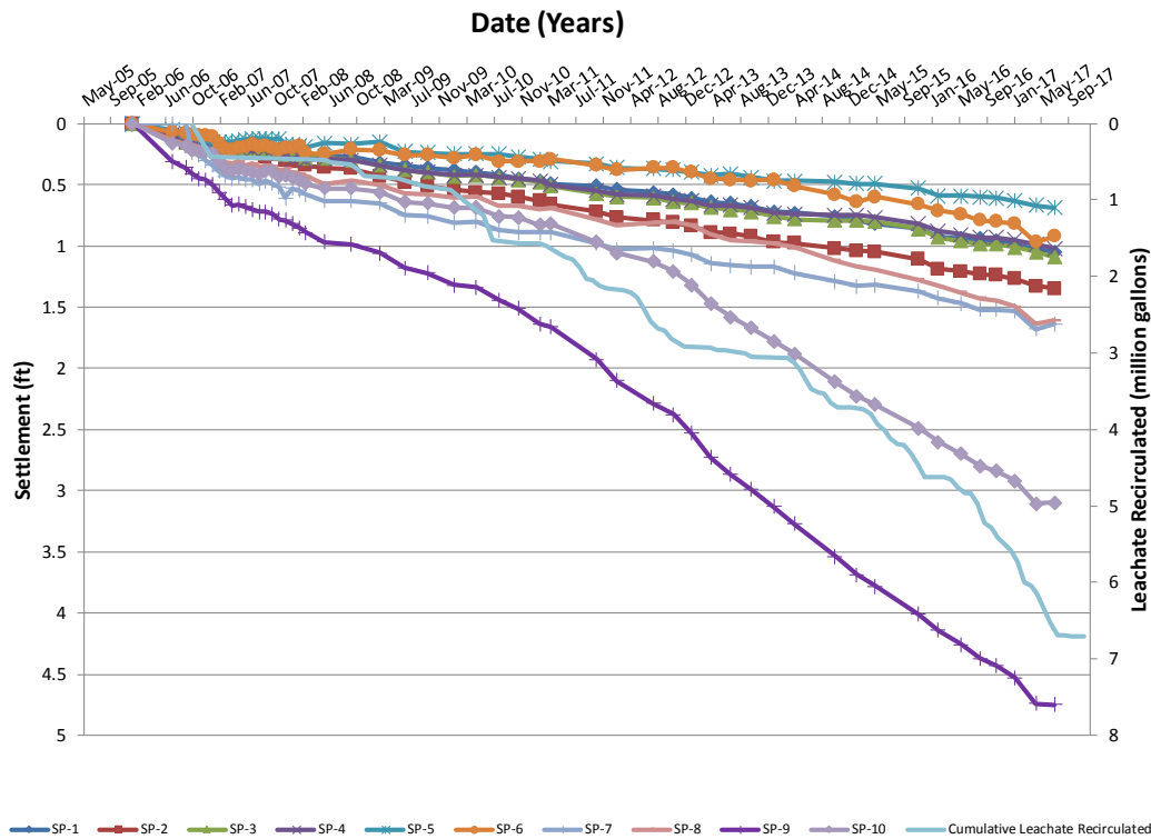
Figure 4-19 Cumulative Settlement
